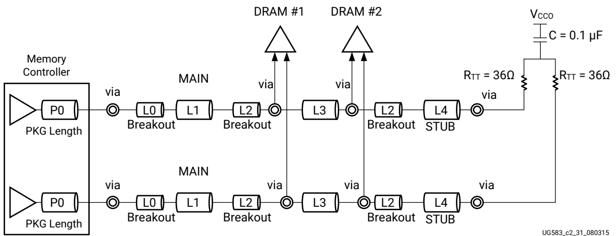
Figure 73: Clock Differential Fly-by Routing for RLDRAM 3 Memory
