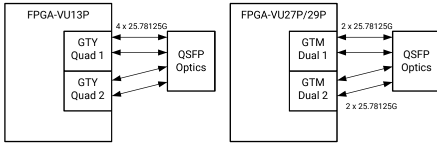
Figure 203: GTY to GTM Transceiver Mapping for 100G Ethernet
