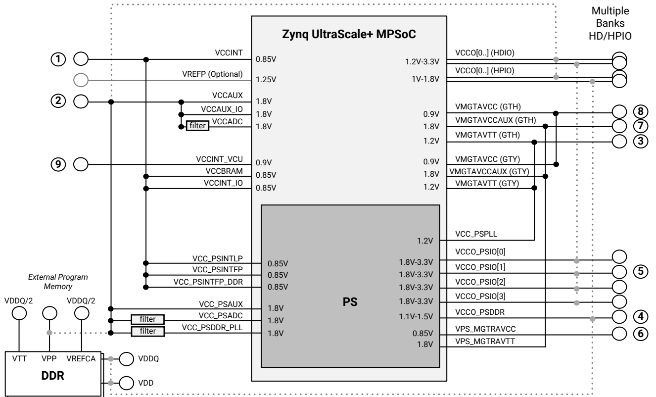
Figure 4: Always On: Cost-Optimized Power Rail Consolidation
