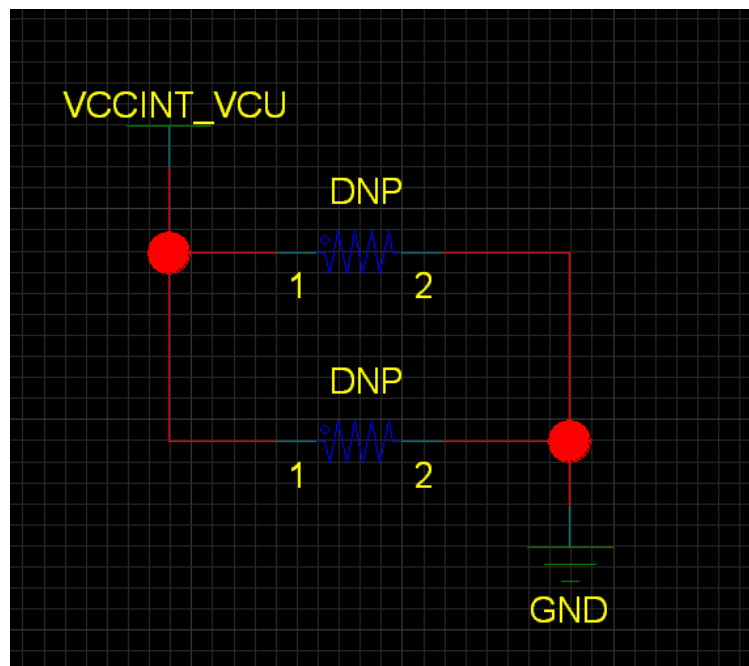
Figure 190: VCCINT_VCU Connection Options for CG/EG/EV Migration (Schematic)
