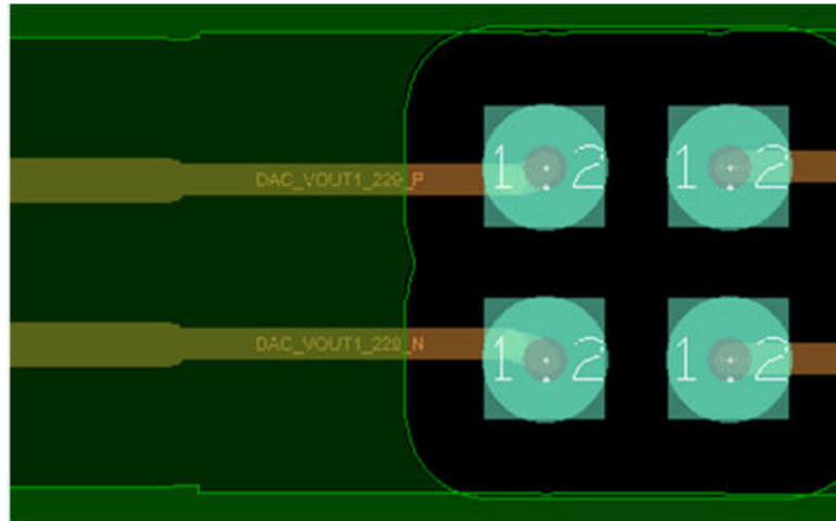
Figure 146: Layer 2 Routing for AC Coupling Capacitor Inputs and Outputs
