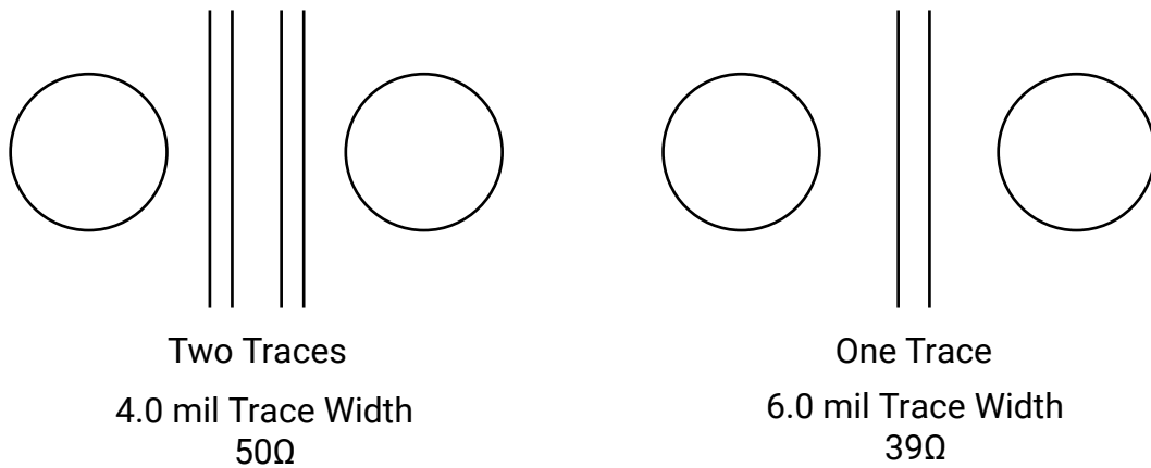
Figure 11: UltraScale Device Breakout Single-Ended Routing Options
