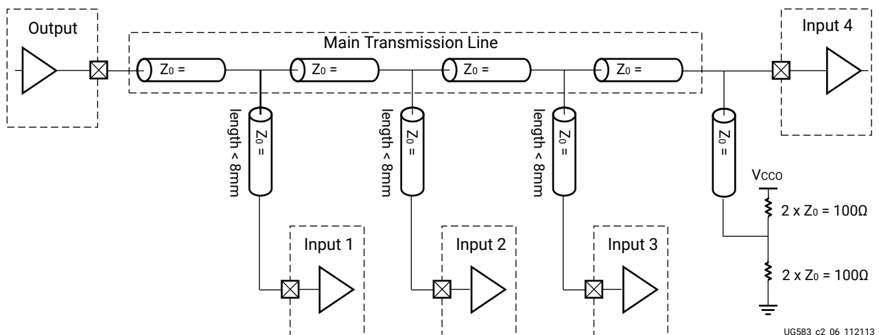
Figure 209: Basic Multi-Drop Topography
