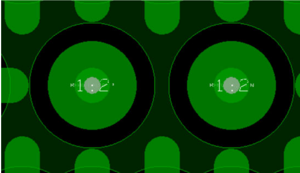
Figure 134: Circular Antipad
