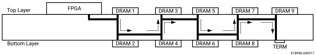
Figure 32: Address/Command/Control Topology for DDR4 SDRAM Clamshell
