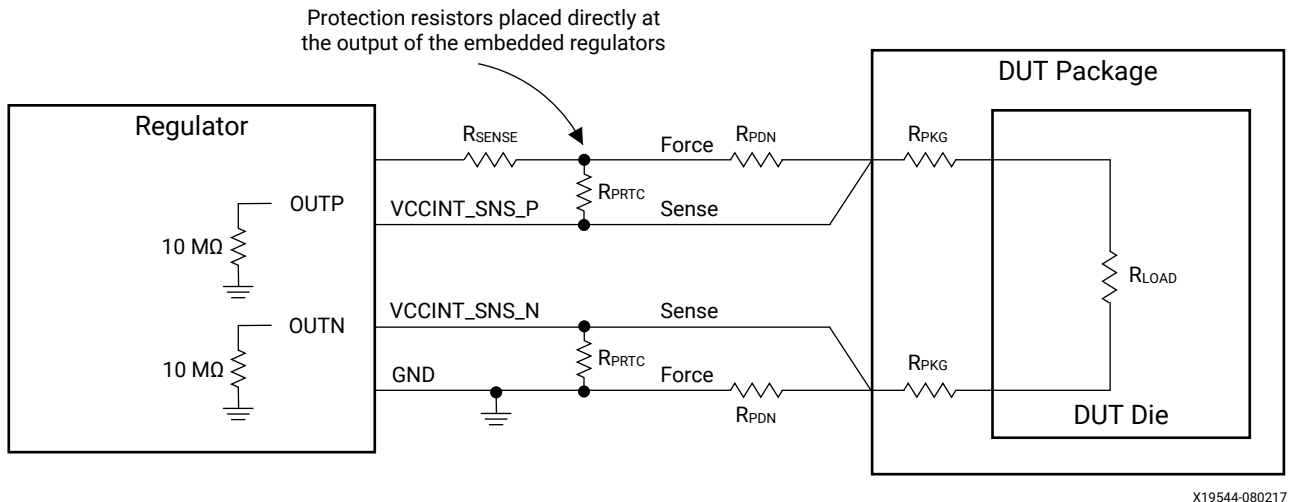
Figure 152: Recommended Sense Line Circuitry
