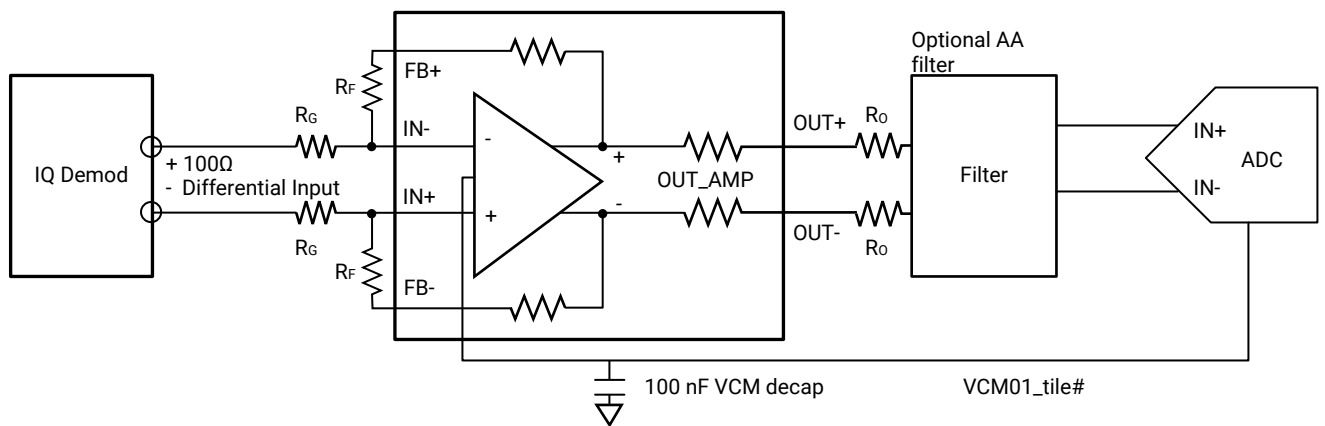
Figure 125: Typical ADC DC Coupling Configuration
