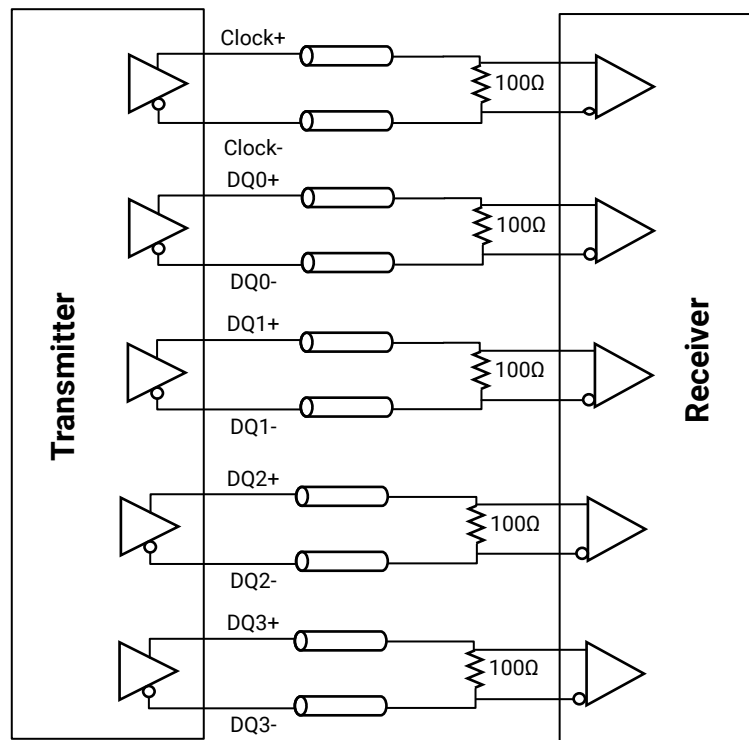
Figure 160: MIPI D-PHY Transmitter and Receiver Paths
