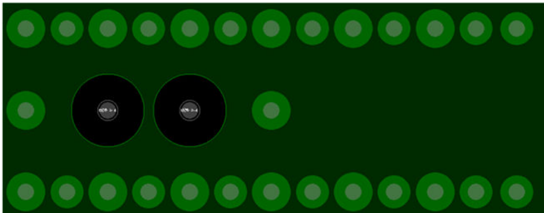
Figure 143: Layer 5 in BGA Area for DACs/ADCs
