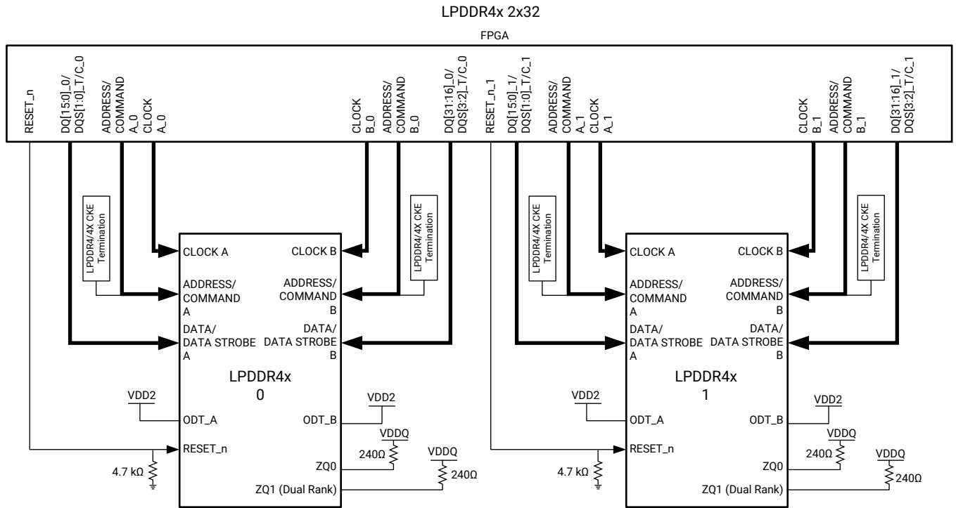
Figure 113: Connections for a 2x32 LPDDR4x Interface
