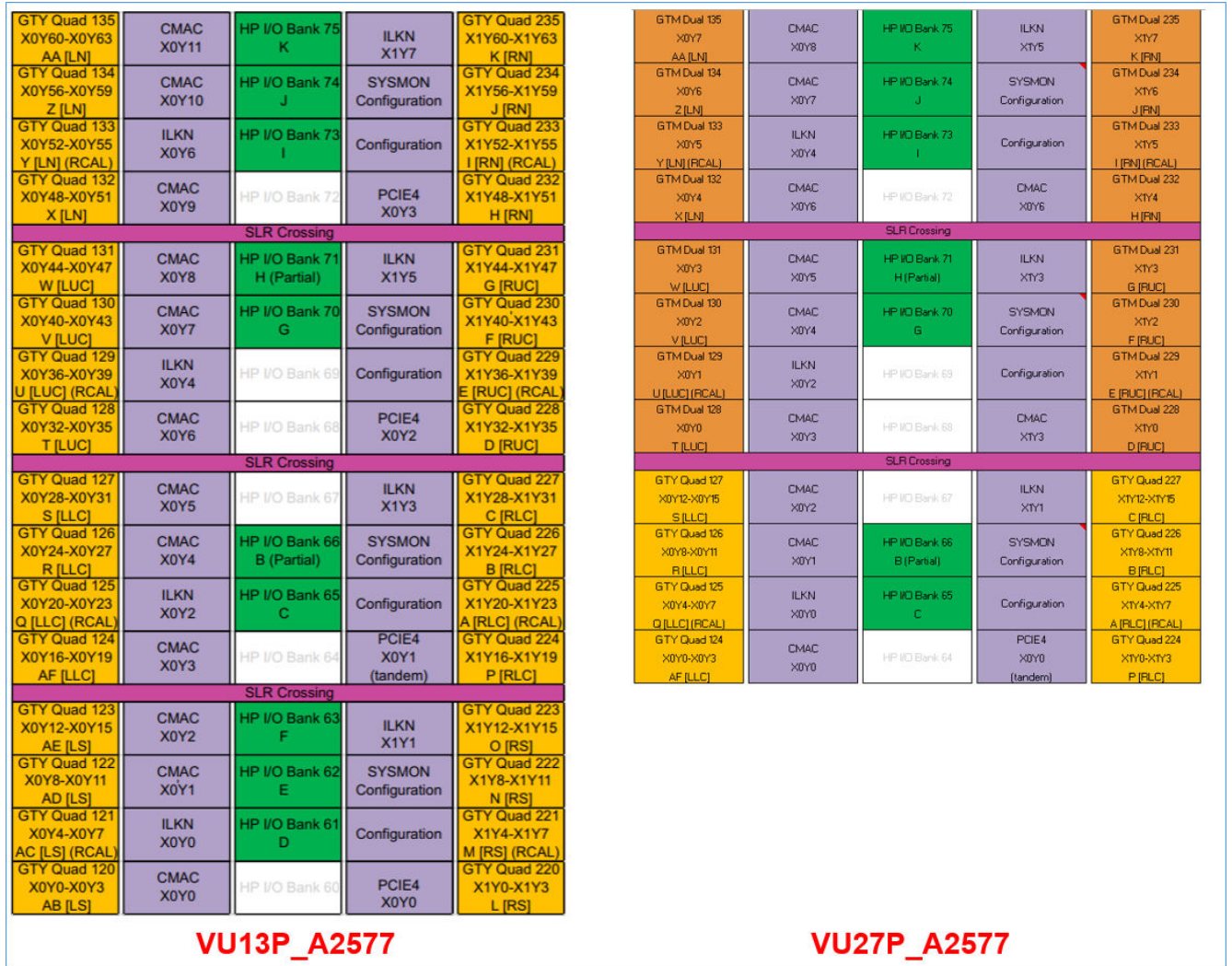
Figure 197: Unavailable SLR on VU27P
