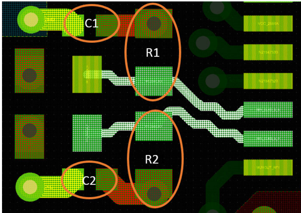
Figure 124: PLL Layout
