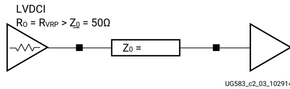
Figure 207: "Weak Driver" Unidirectional, Point-to-Point Topography
