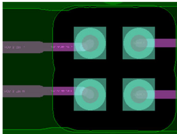
Figure 147: Layer 4 Routing for AC Coupling Capacitor Inputs and Outputs
