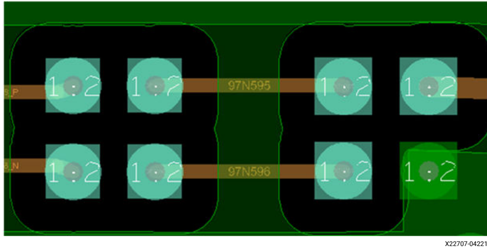
Figure 148: Layer 2 Between AC Capacitors and Baluns
