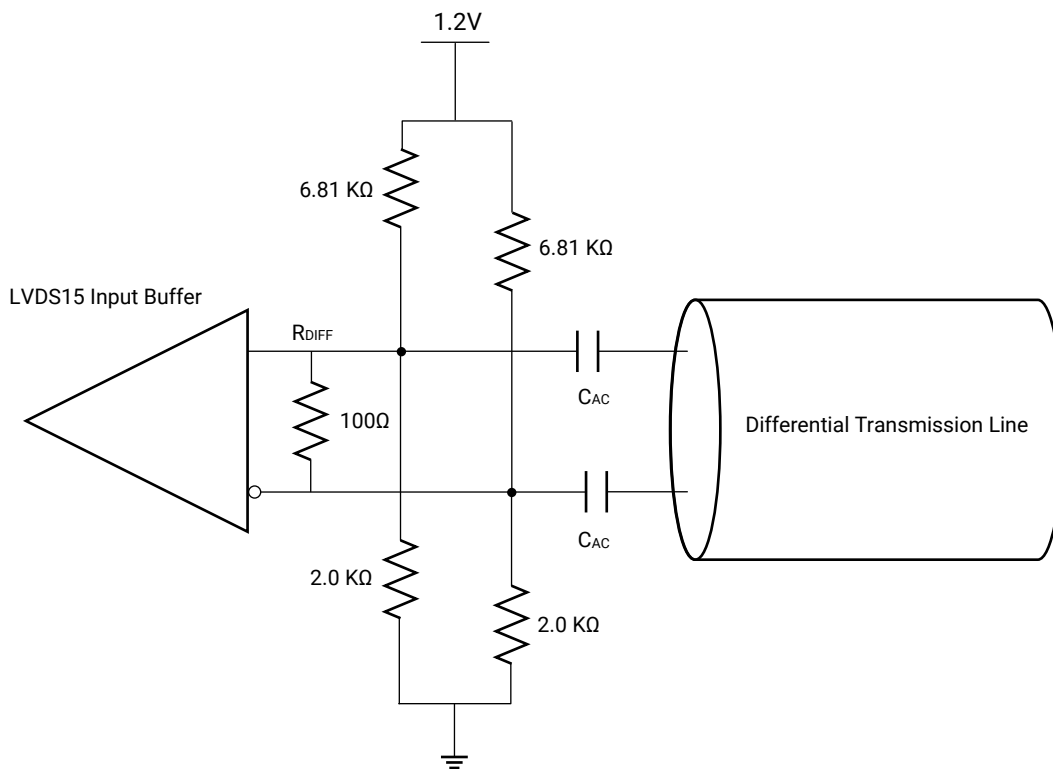
Figure 89: AC-Coupled with DC-Biased Differential Clock Input
