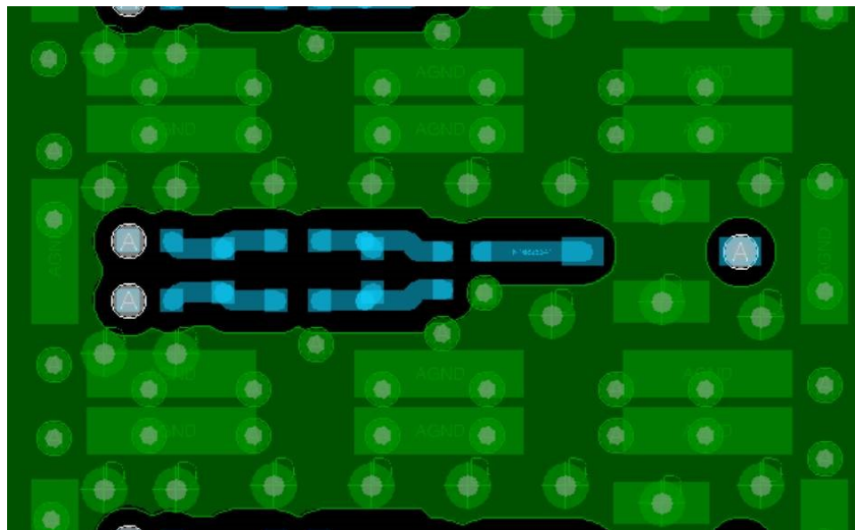
Figure 122: Balun Isolation with GND Stitching and GND Plane
