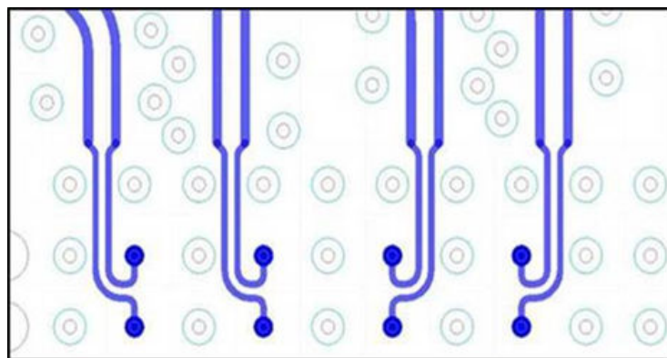
Figure 126: Differential Breakout Example
