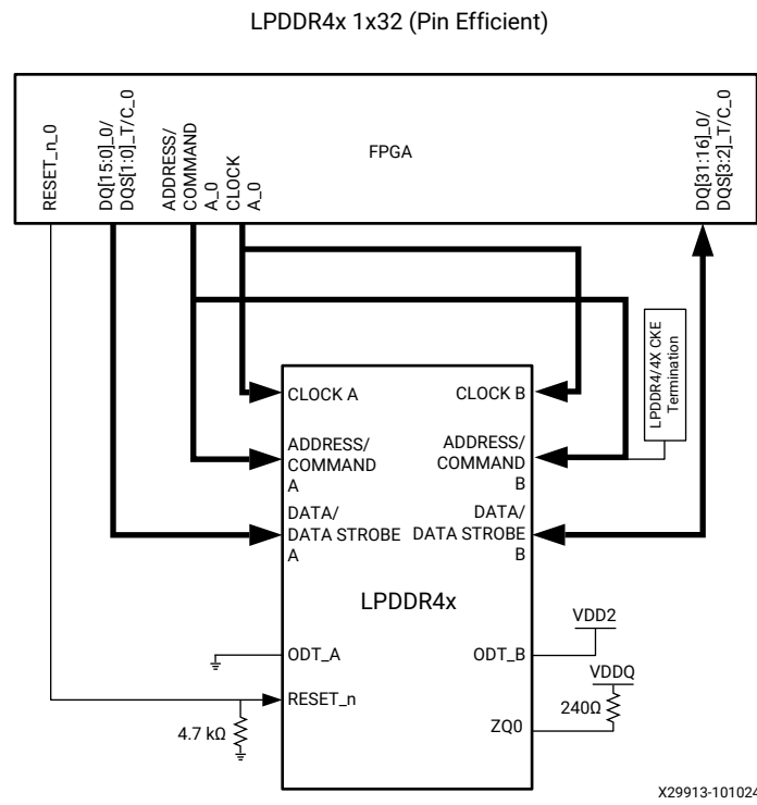
Figure 119: Connections for a Pin Efficient 1x32 LPDDR4x Interface
