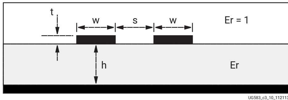
Figure 223: Differential Microstrip
