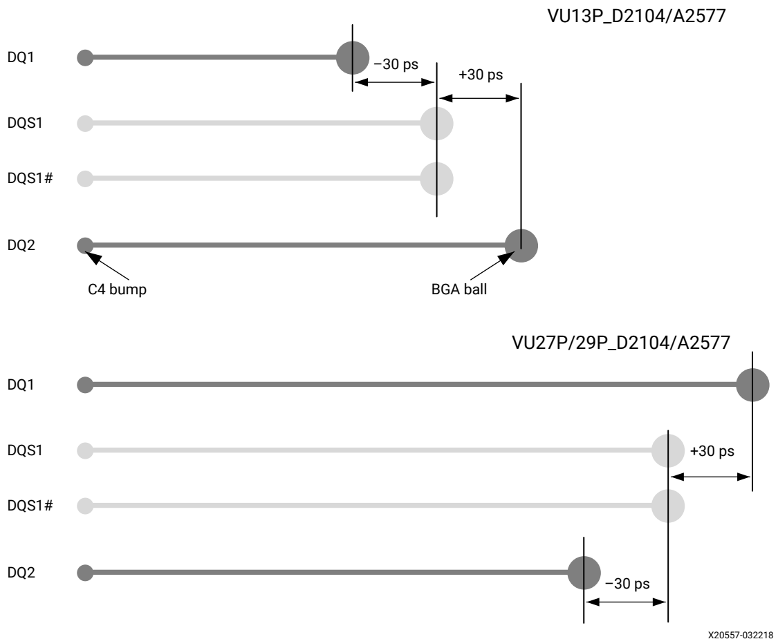
Figure 196: Skew Illustration Across Devices
