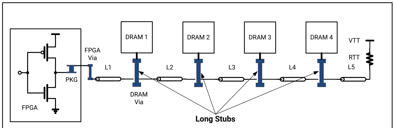
Figure 101: Thicker PCB: Command/Address/Control Bus Conventional Routing
