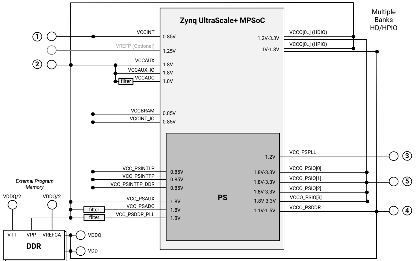
Figure 5: Always On: Cost-Optimized with Only Five Power Regulators (CG or EG Devices)
