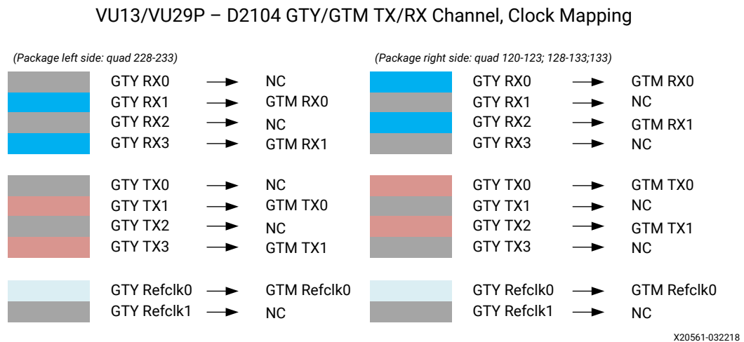
Figure 200: VU13P/VU29P D2104 GTY/GTM TX/RX Channel/Clock Mapping
