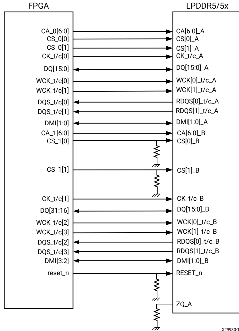
Figure 110: LPDDR5 2x16 Single/Dual Rank
