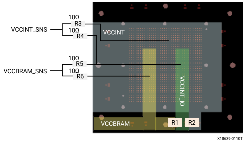
Figure 178: Reference Layout to Support VCCINT/VCCINT_IO/VCCBRAM Connection Matrix
