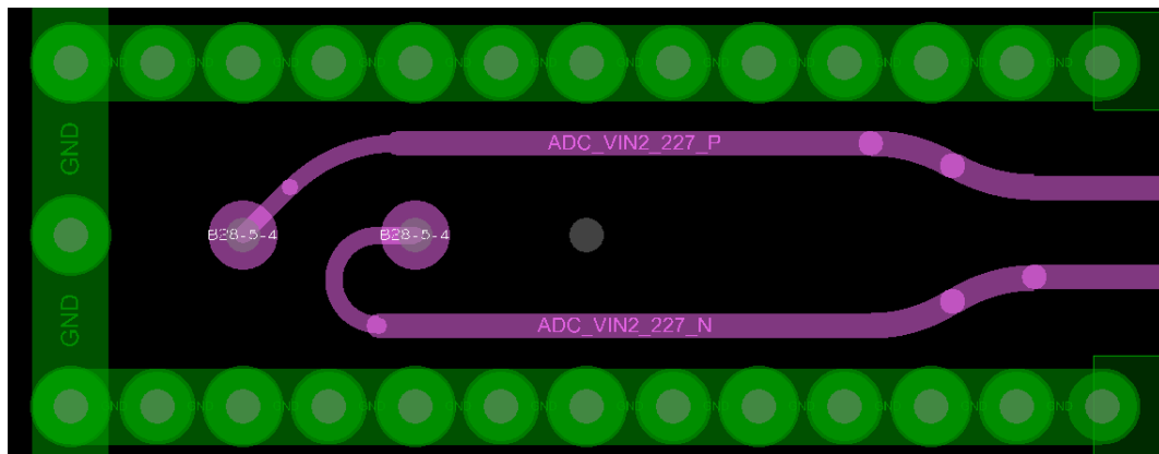
Figure 142: Layer 4 in BGA Area for DACs/ADCs
