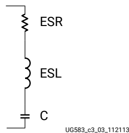
Figure 216: Parasitics of a Real, Non-Ideal Capacitor
