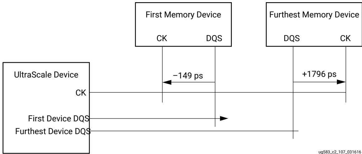
Figure 14: Interpretation of CK to DQS Skew Specification
