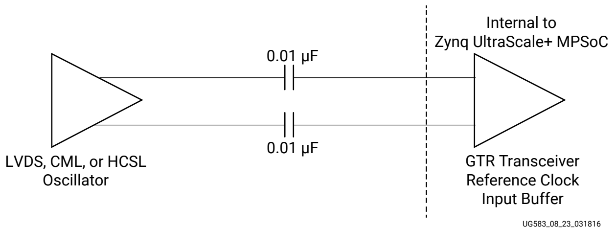
Figure 158: Interfacing an LVDS, CML, or HCSL Oscillator to the Zynq UltraScale+ MPSoC PS-GTR Transceiver Reference Clock Input
