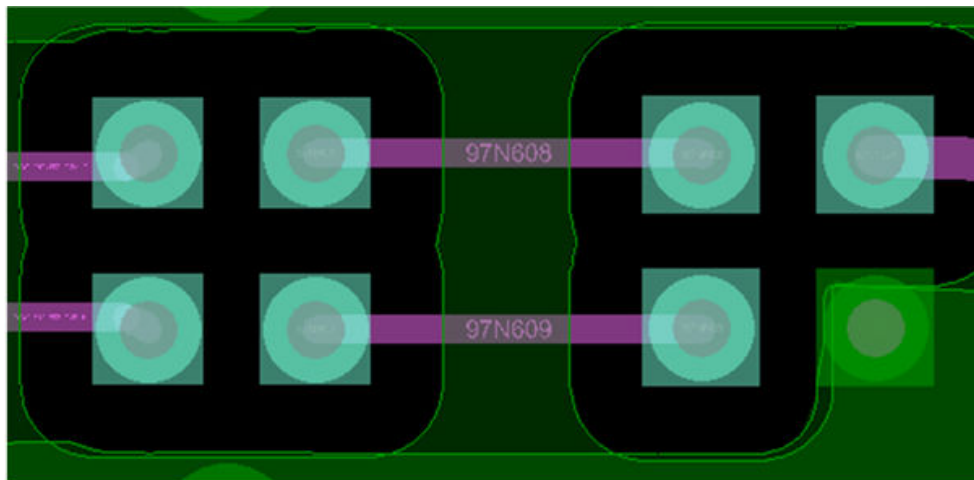
Figure 149: Layer 4 Between AC Capacitors and Baluns
