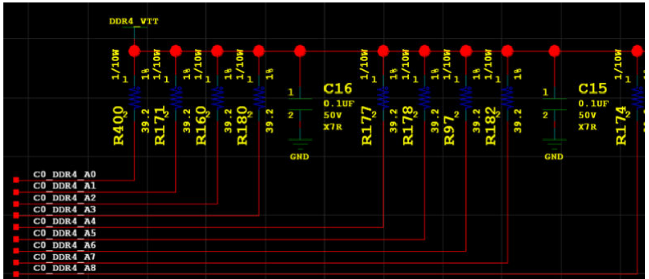
Figure 96: Schematic Example of VTT Resistor and Capacitor Connections
