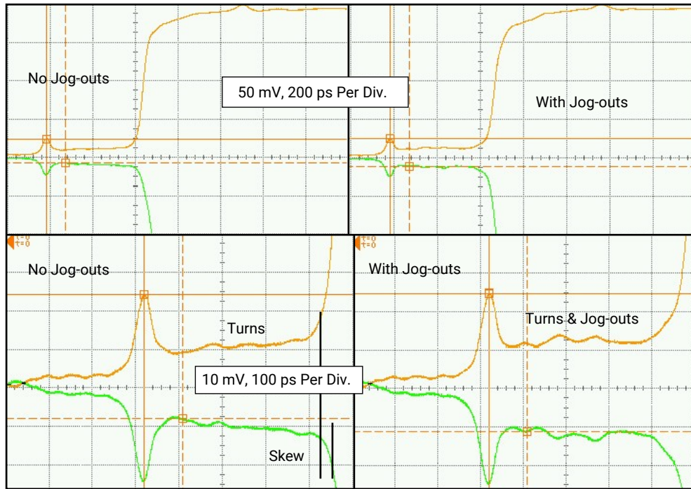
Figure 246: Measured TDR of 45 Degree Bends with and without Jog-Outs
