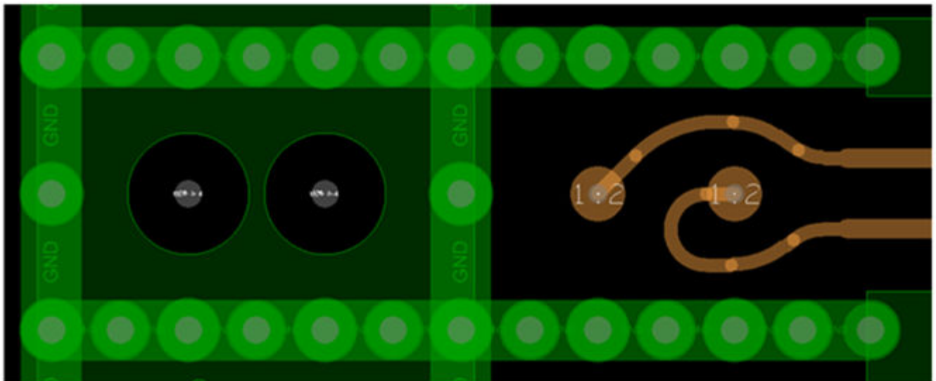
Figure 140: Layer 2 in BGA Area for DACs/ADCs
