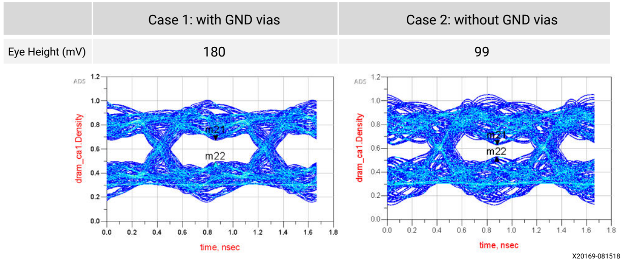
Figure 21: Simulations With and Without Ground Stitching Vias
