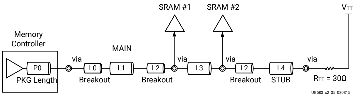
Figure 79: Address and Command Fly-by Routing and Termination for QDR II+ SRAM
