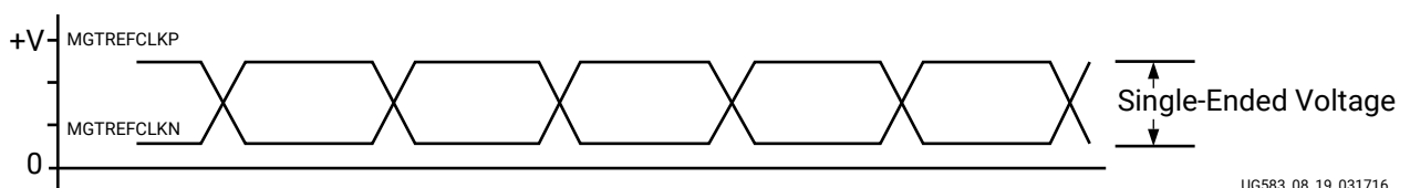
Figure 154: Single-Ended Clock Input Voltage Swing, Peak-to-Peak
