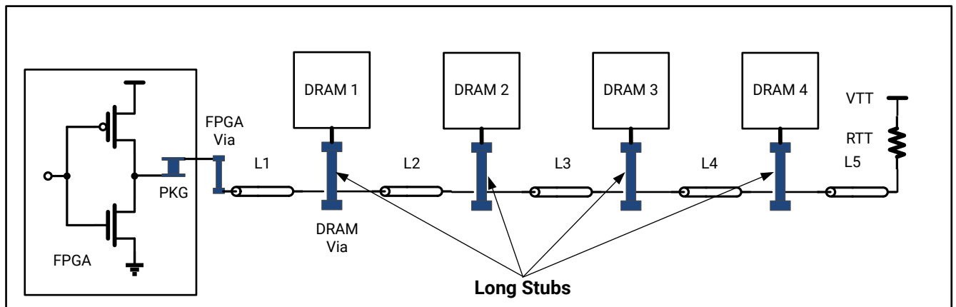
Figure 28: Thicker PCB: Command/Address/Control Bus Conventional Routing
