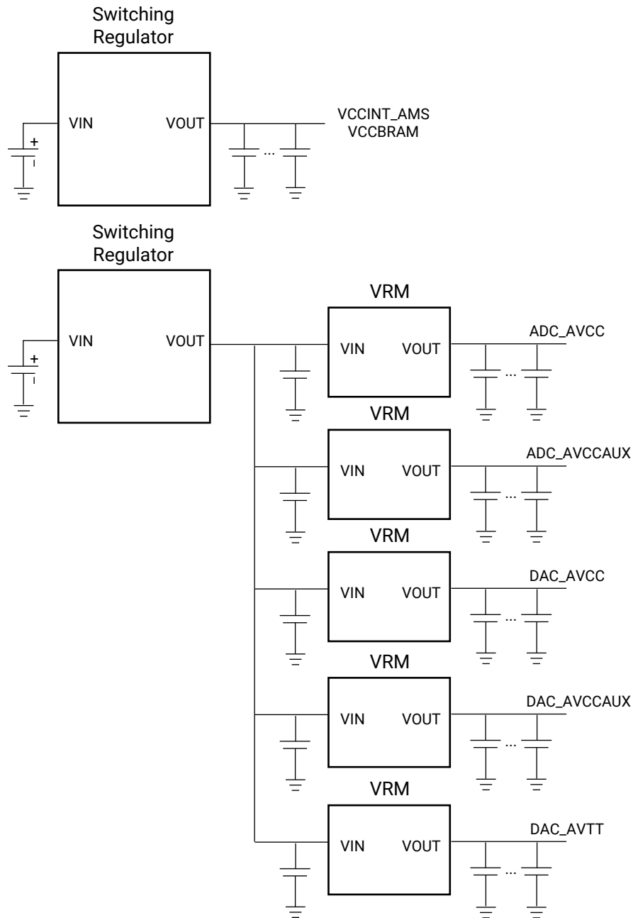
Figure 150: Power Regulation for Analog Supplies
