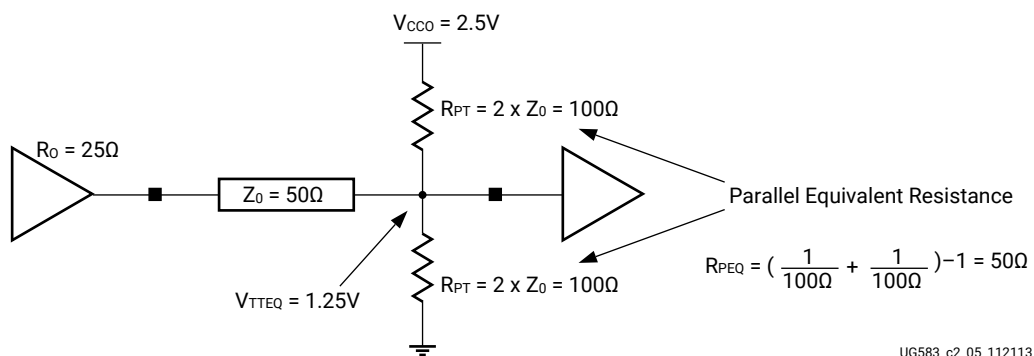
Figure 208: Thevenin Parallel Termination
