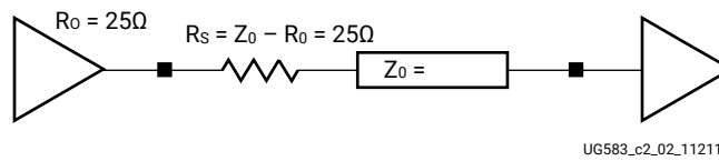
Figure 206: DCI-Controlled Impedance Driver Unidirectional, Point-to-Point Topography
