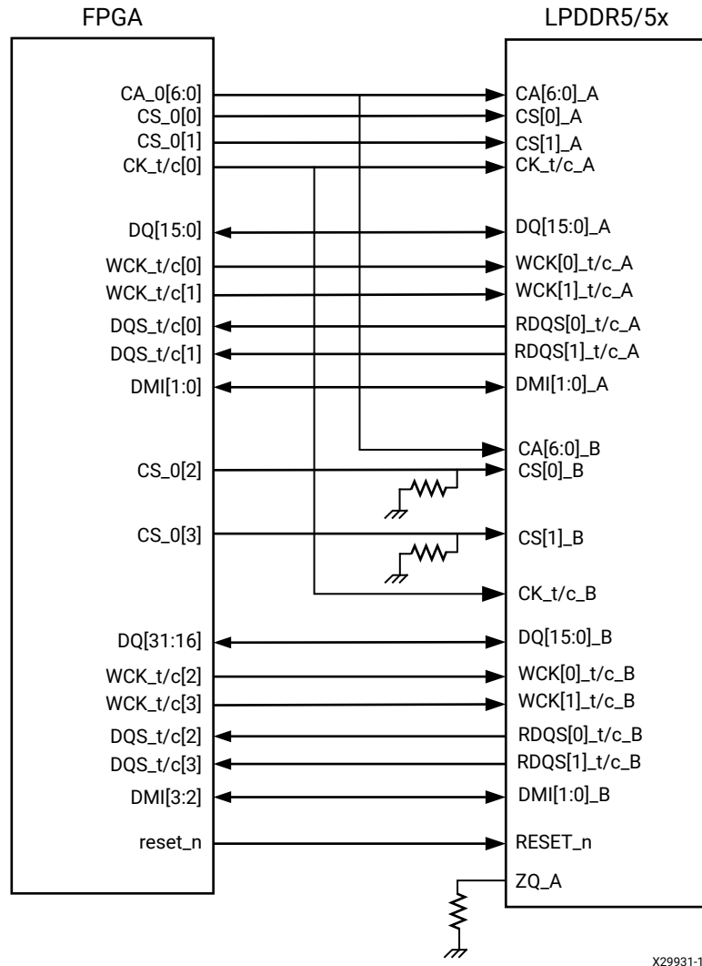
Figure 111: LPDDR5 1x32 Single/Dual Rank
