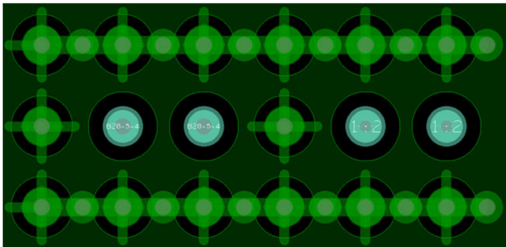
Figure 139: Layer 1 in BGA Area for DACs/ADCs
