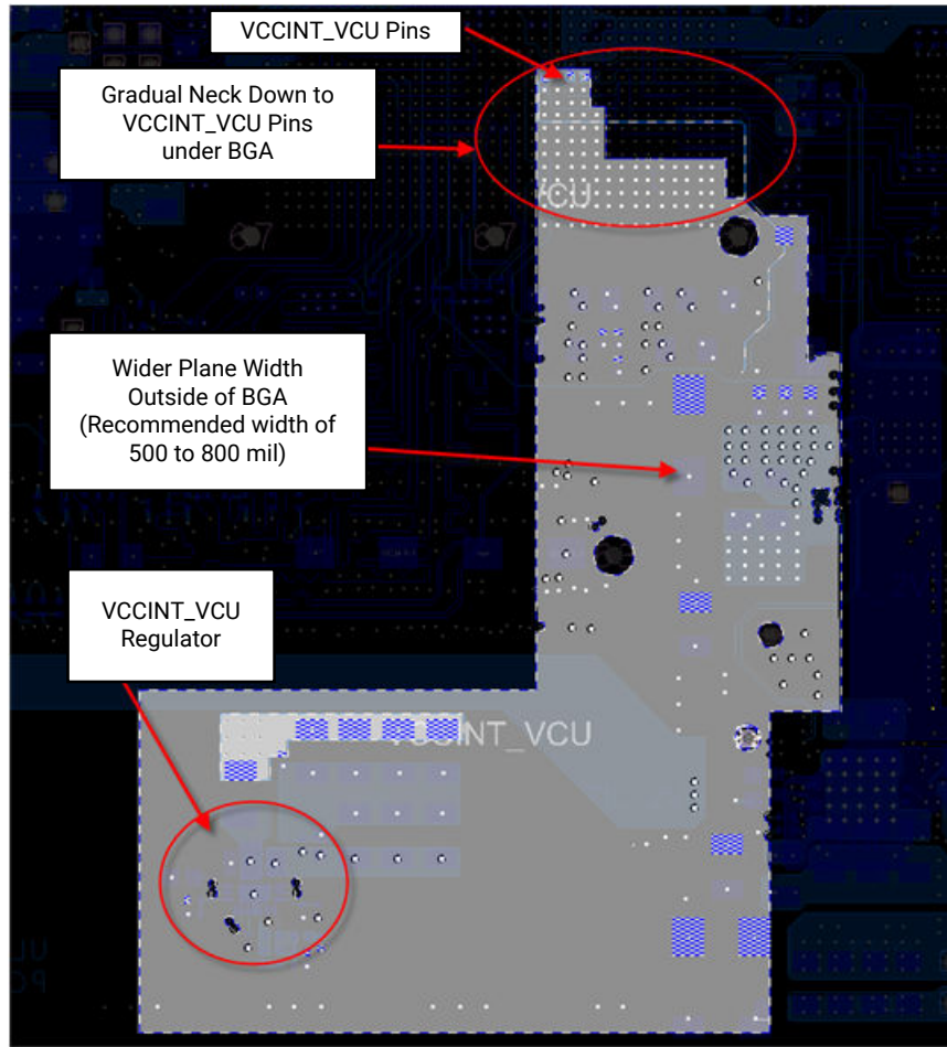
Figure 3: Example Plane Layout for V CCINT_VCU
