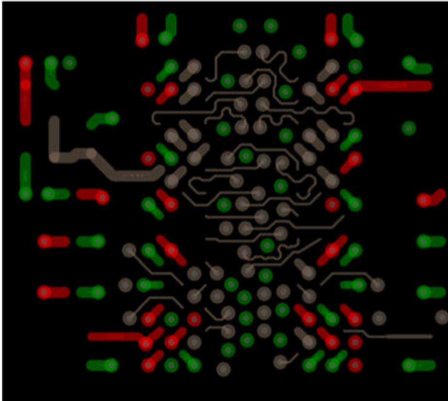
Figure 94: Example of Ground Stitching (Clamshell) Red: Power, Green: Ground
