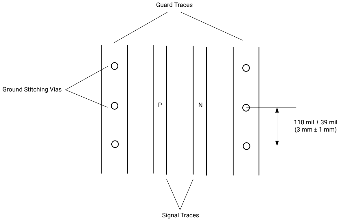
Figure 128: Close View of Guard Traces and Ground Stitching
