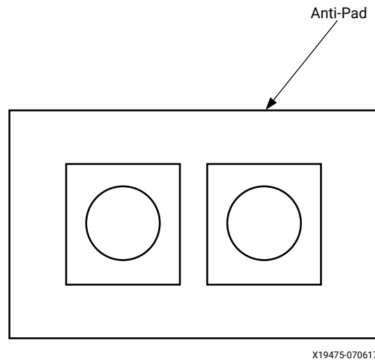
Figure 151: Decoupling Capacitor Antipad
