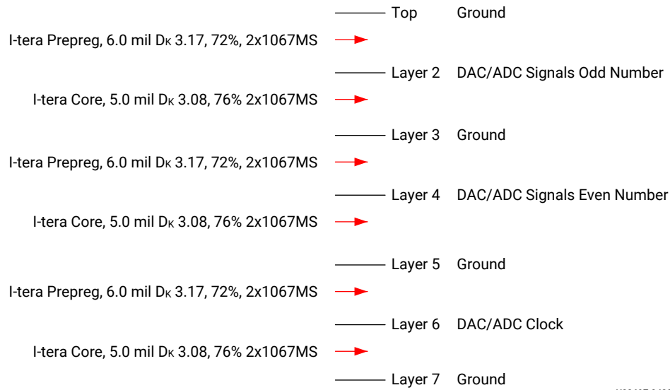
Figure 138: PCB Stackup
