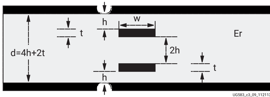
Figure 222: Centered Broadside-Coupled Stripline
