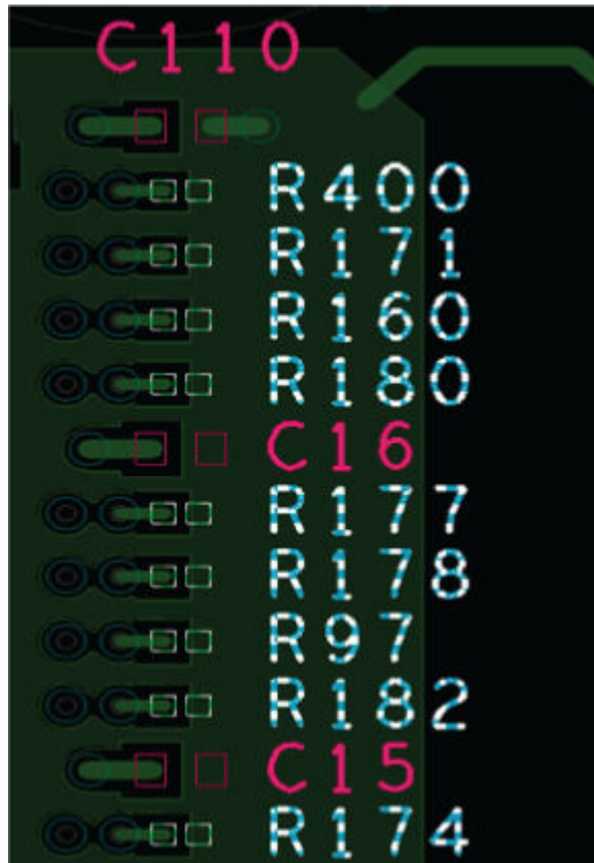
Figure 97: Example of V_{TT} Termination Placement
