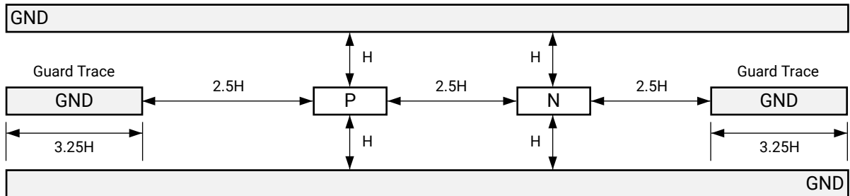
Figure 129: Cross-Section of Guard Traces
