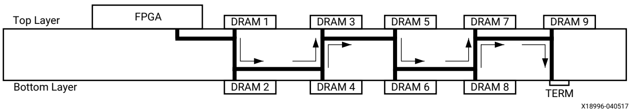
Figure 105: Address/Command/Control Topology for DDR4 SDRAM Clamshell
