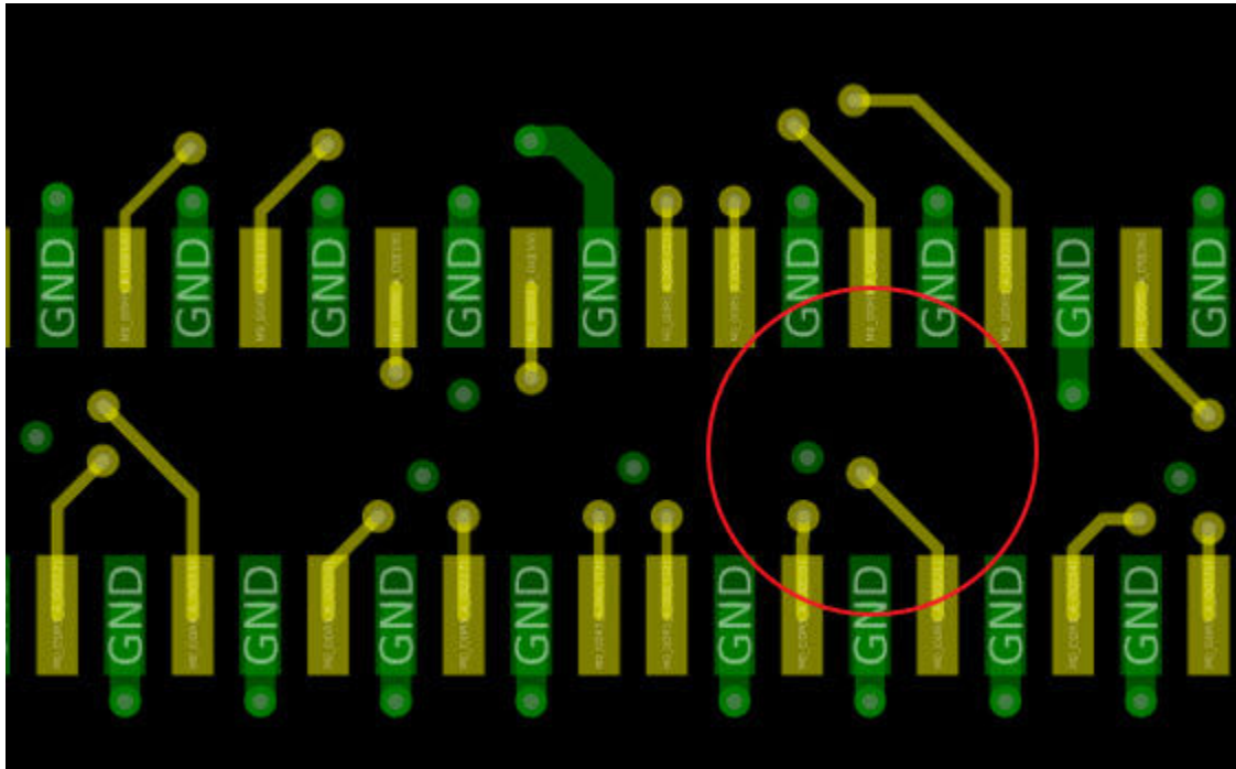
Figure 98: Ground Via Radius
