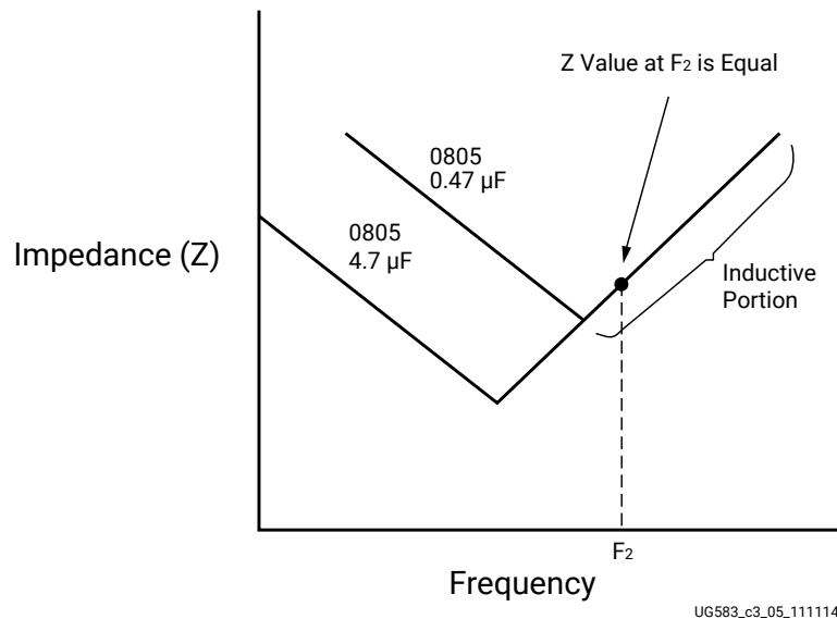
Figure 218: Effective Frequency Example
