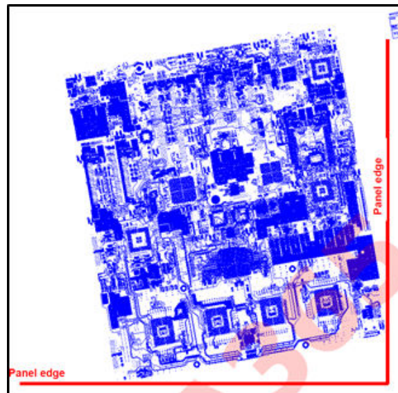
Figure 130: Rotated Panel to Compensate for Glass Non-Homogeneity
