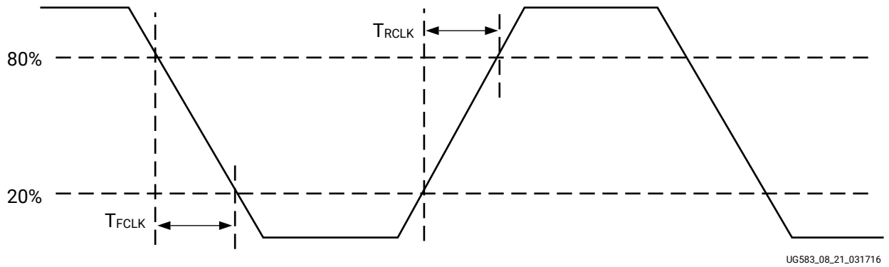
Figure 156: Rise and Fall Times
