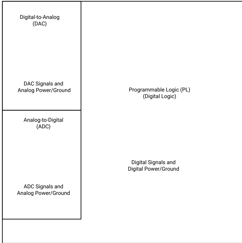
Figure 121: XCZU28DR-FFVE1156 Floorplan
