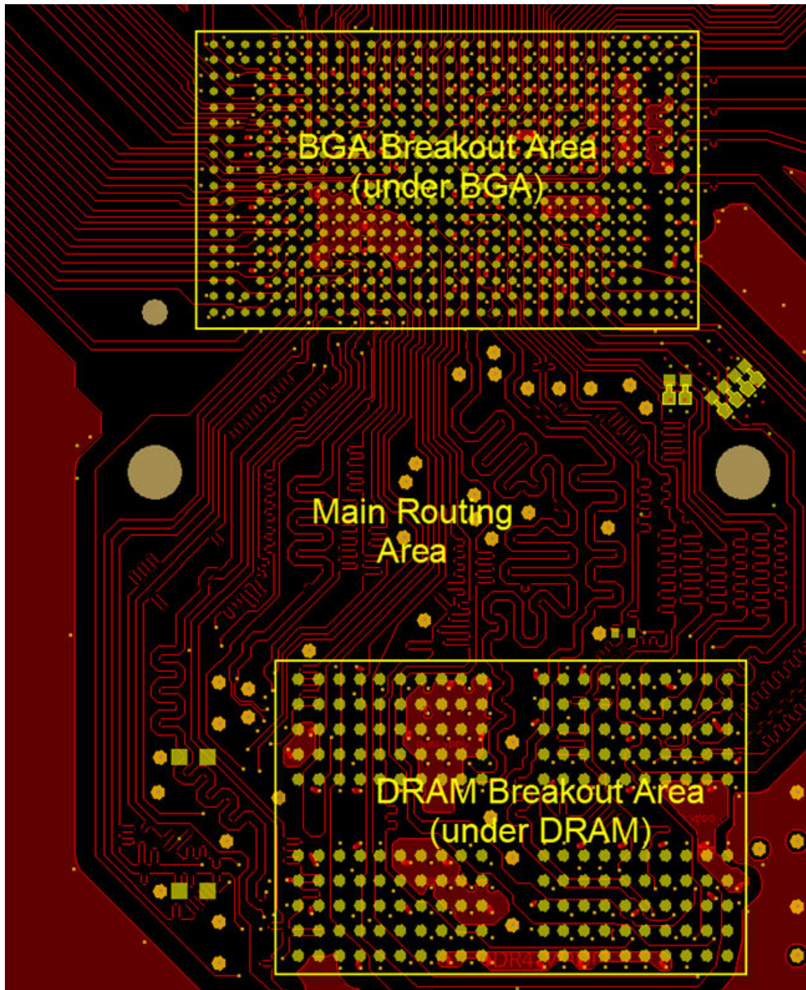
Figure 60: Reference PCB with Routing Areas Denoted
