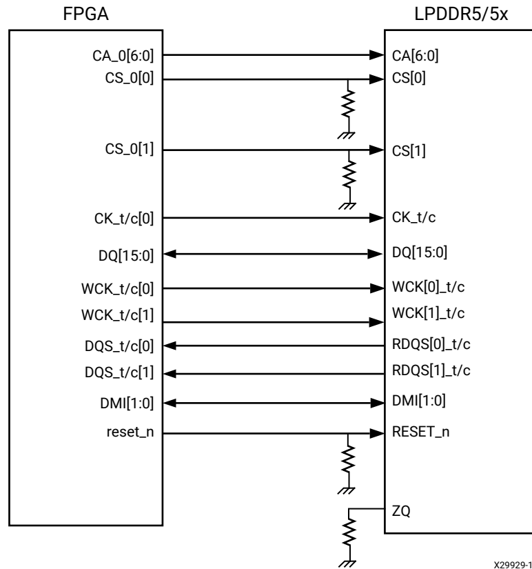
Figure 109: LPDDR5 1x16 Single/Dual Rank
