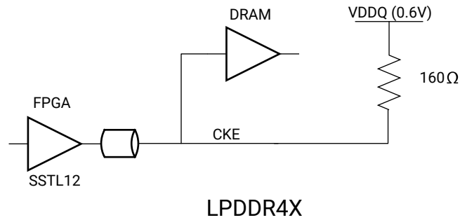
Figure 112: LPDDR4X CKE Termination
