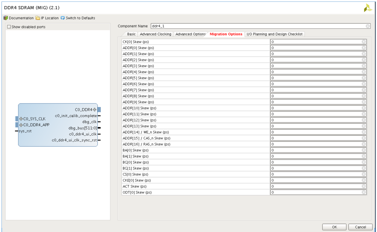
Figure 193: Entering the Pin Delay Differences for Migration
