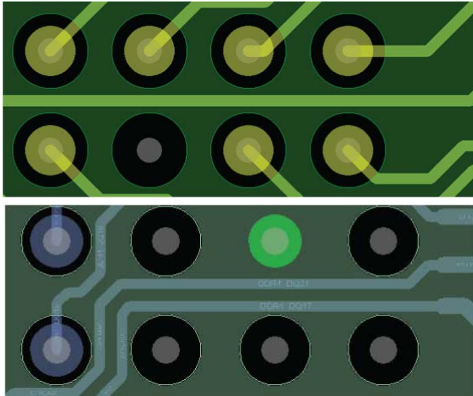
Figure 92: Breakout Region Routing
