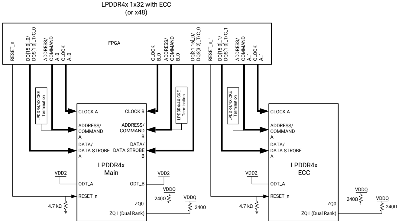
Figure 114: Connections for a 1x32 (or x48) with ECC LPDDR4x Interface
