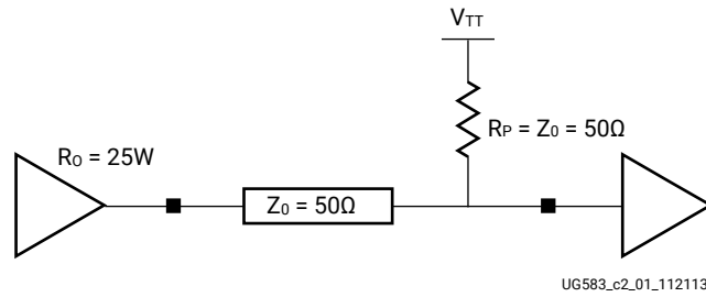
Figure 205: Series-Terminated Unidirectional, Point-to-Point Topography
