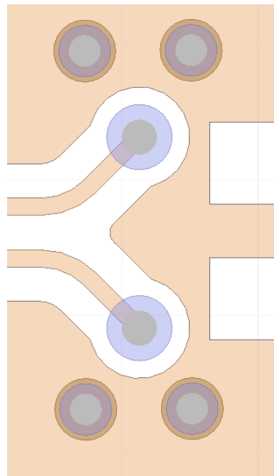
Figure 132: Via Configuration for Signal Layer Transition
