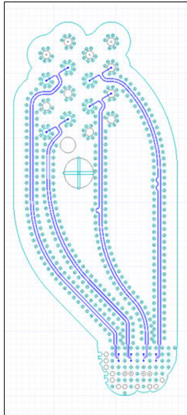
Figure 127: Example of Ground Stitching around Signal Pairs
