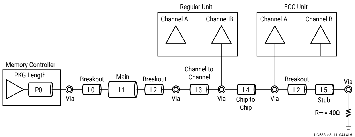
Figure 53: CS0/CS1 Routing for LPDDR4 with ECC
