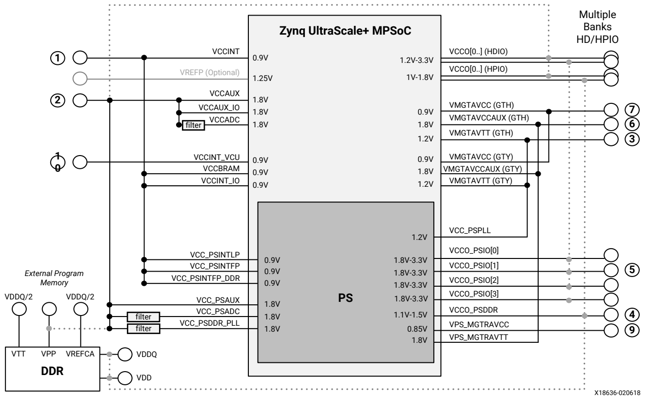
Figure 7: Always On: PL Performance-Optimized Rail Consolidation
