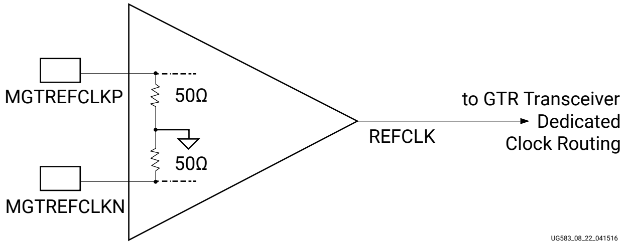
Figure 157: MGTREFCLK Input Buffer Details
