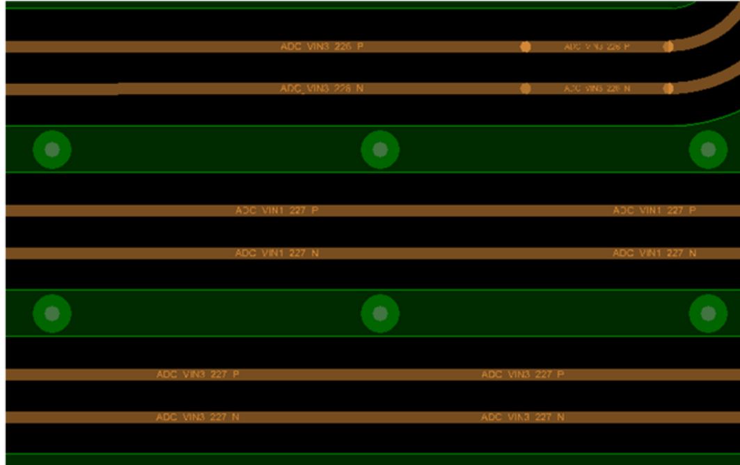
Figure 145: Guard Traces along Trace Route Length
