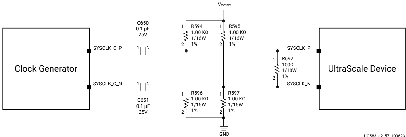
Figure 15: System Clock
