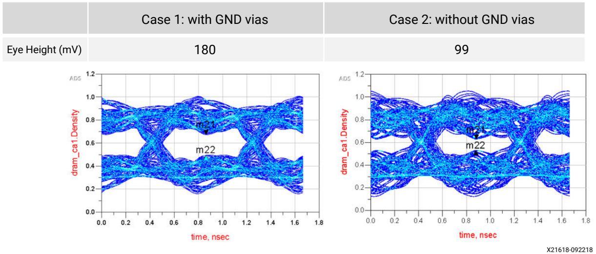
Figure 95: Simulations With and Without Ground Stitching Vias
