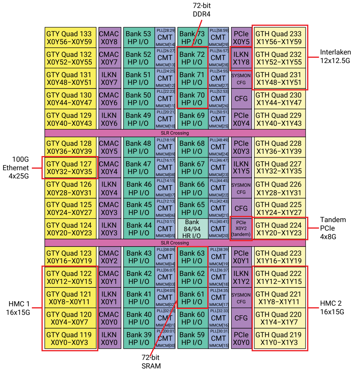
Figure 182: Example VU190 Design Floorplan
