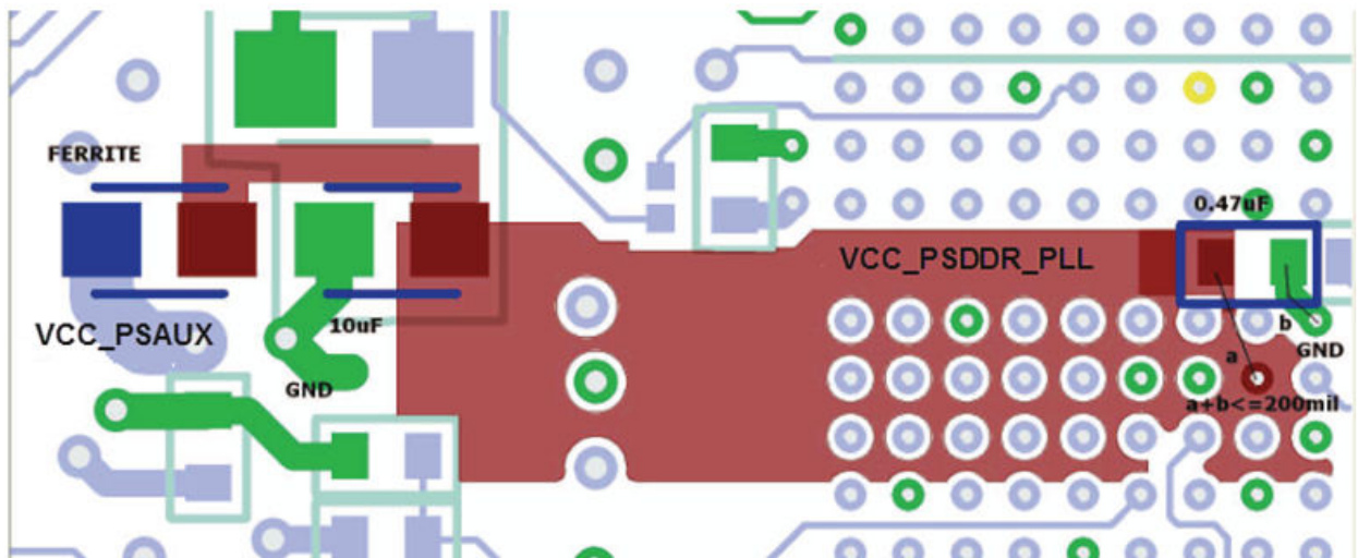
Figure 2: Filtering Circuit Layout
