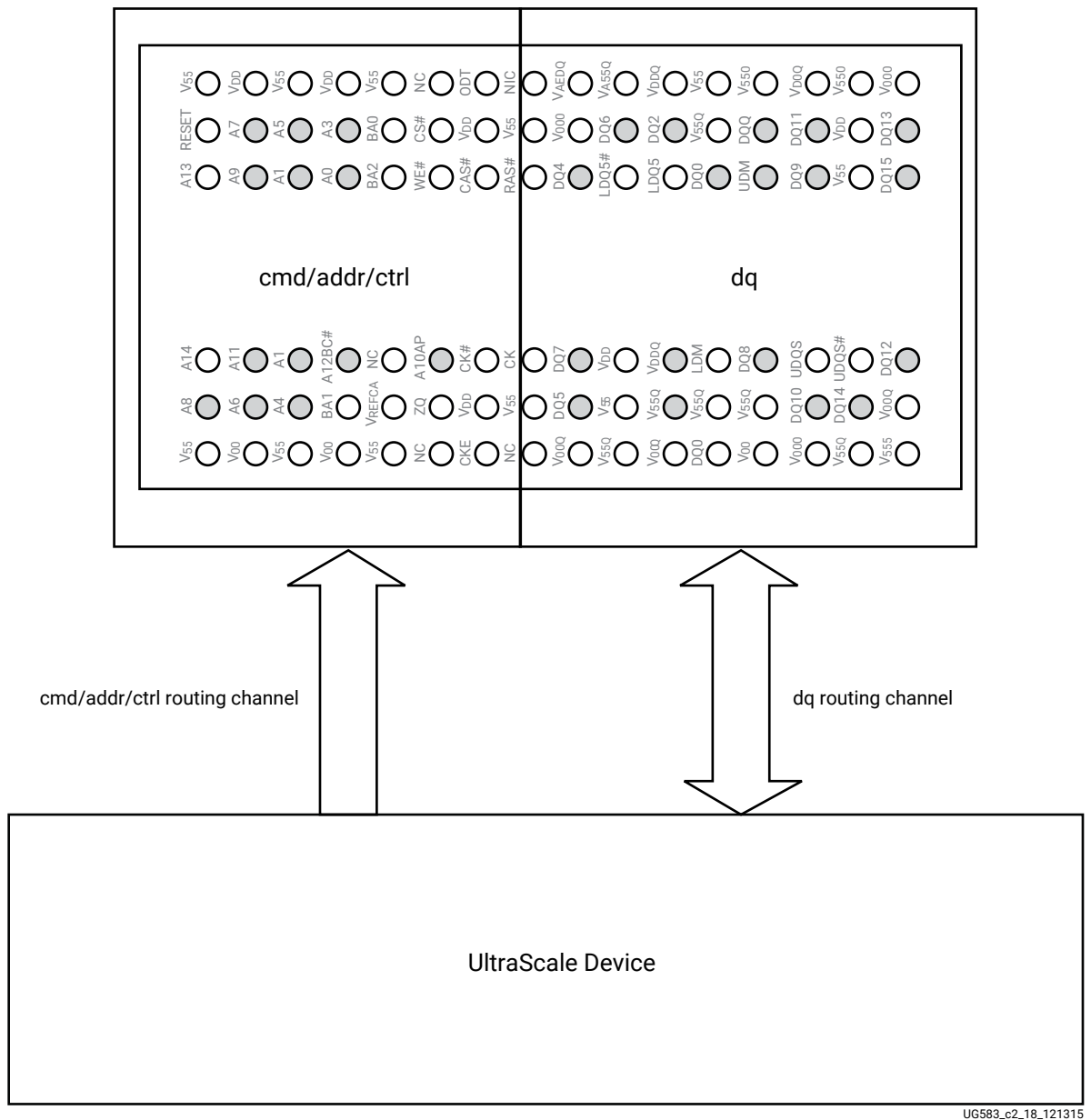
Figure 24: Component Placement Recommendations for One Component
