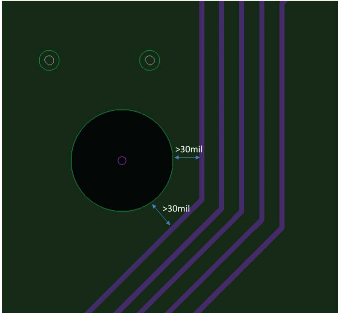
Figure 90: Signal Routing Over Solid Reference Plane
