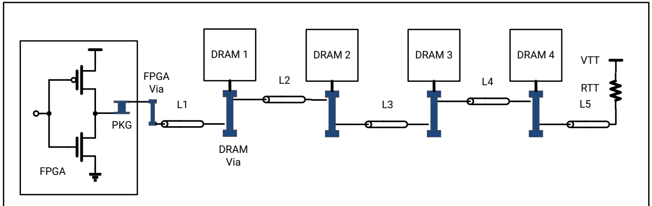
Figure 102: Thicker PCB: Command/Address/Control Bus Stub-Free Routing
