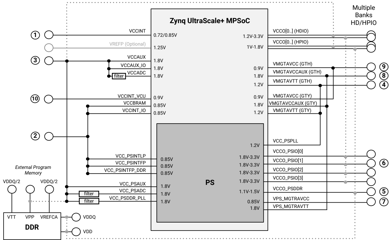
Figure 6: Always On: Power and/or Efficiency-Optimized Power Rail Consolidation for Low-Power Devices
