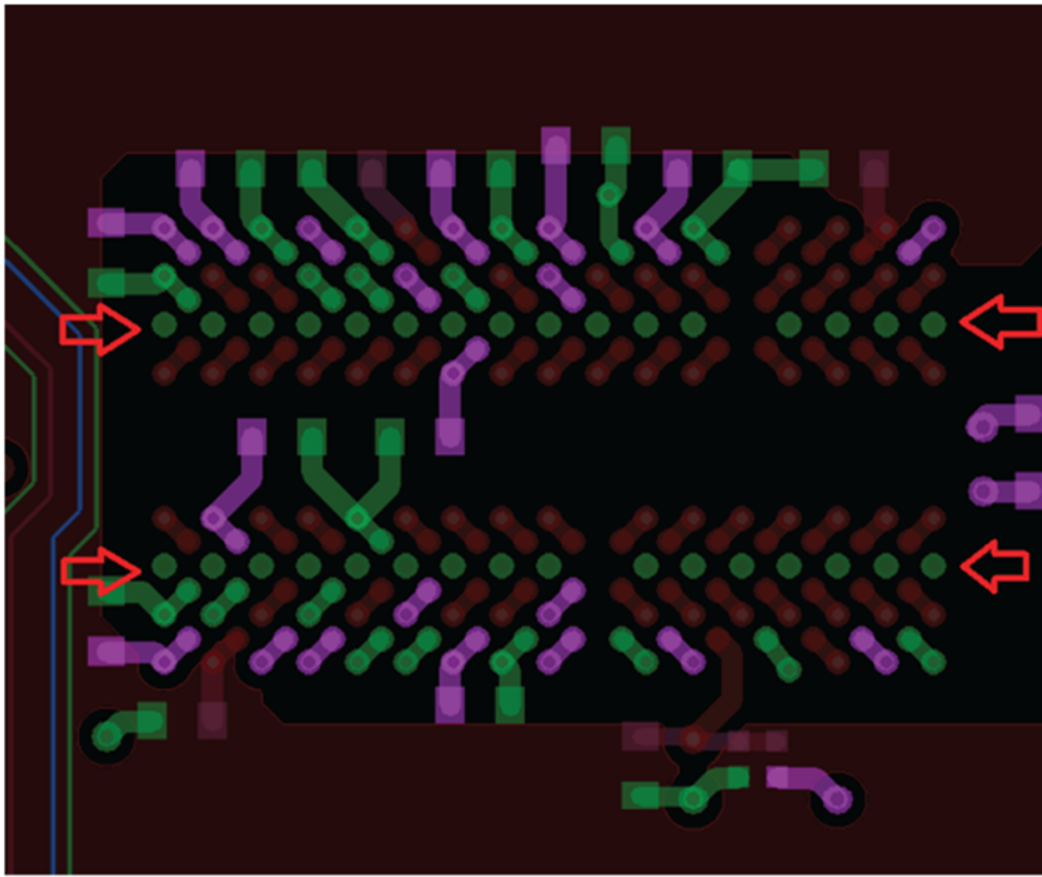
Figure 19: Example of Ground Stitching (Fly-by)
