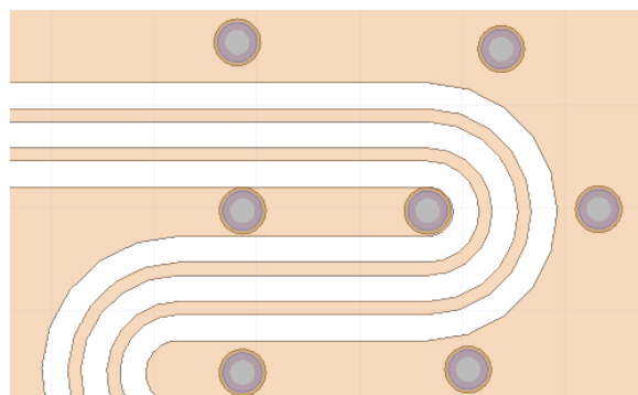
Figure 131: P/N Trace Pair with 180-Degree Bend
