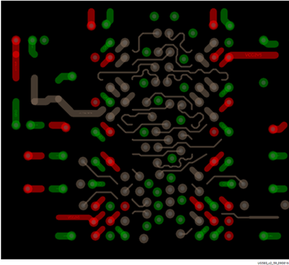
Figure 20: Example of Ground Stitching (Clamshell) Red: Power, Green: Ground
