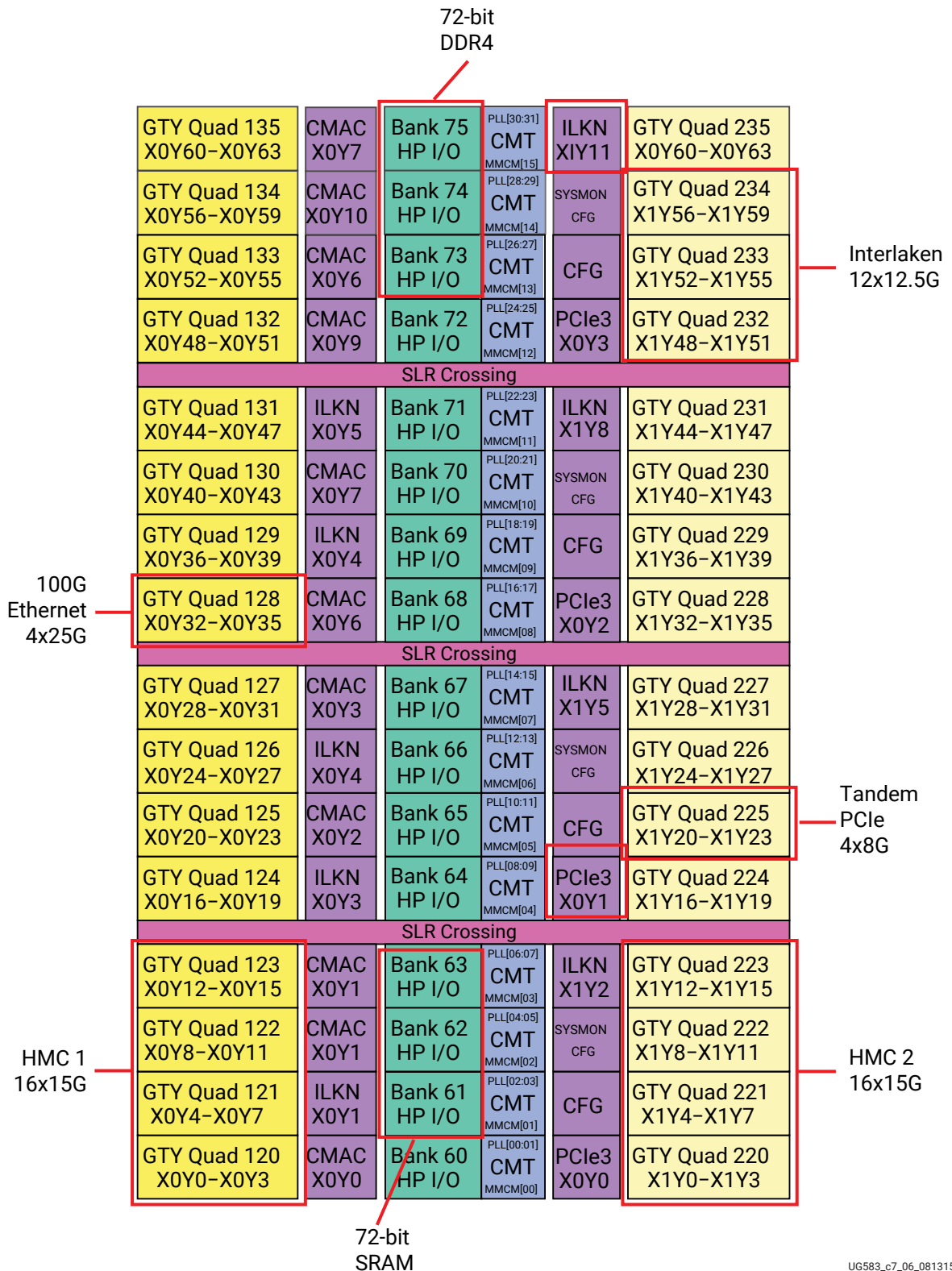
Figure 183: VU13P Floorplan for Migration from VU190
