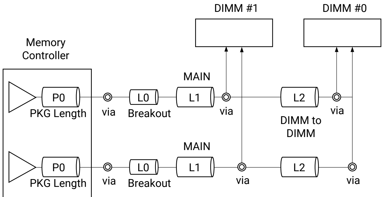
Figure 45: DQ Fly-by Routing for DDR3/DDR4 DIMM Topology
