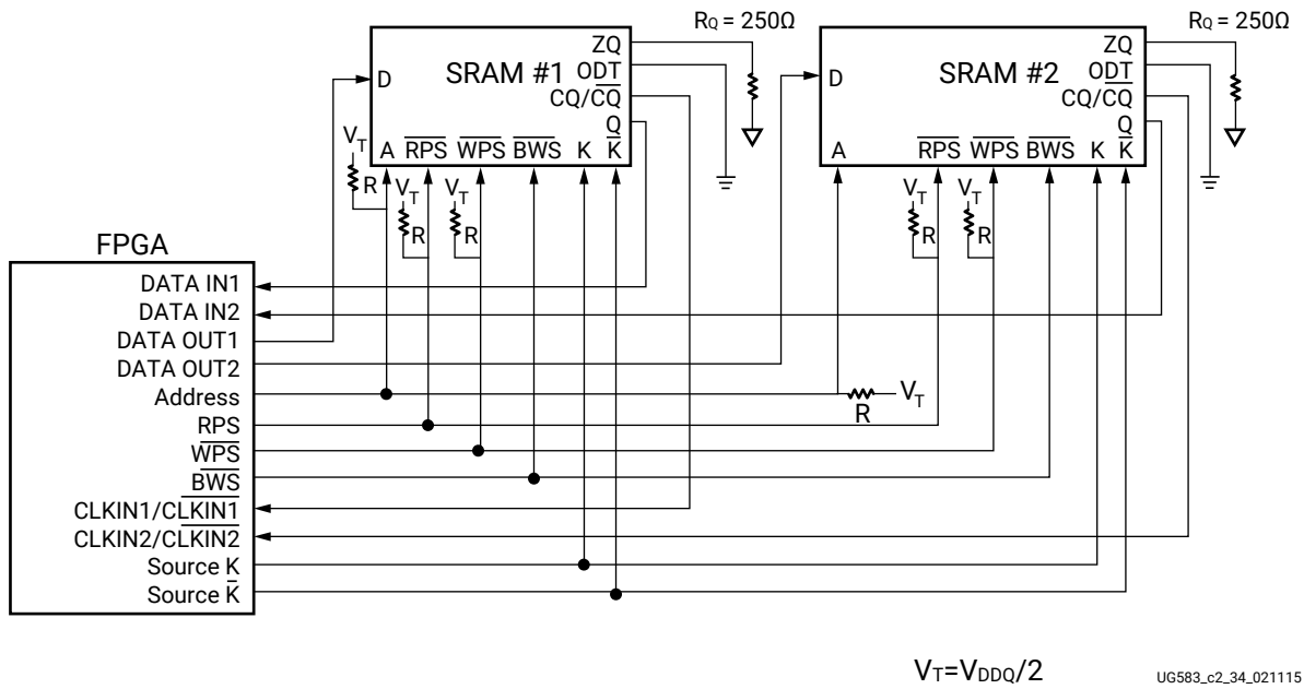
Figure 77: Design Example for QDR II+ SRAM Devices with Width Expansion
