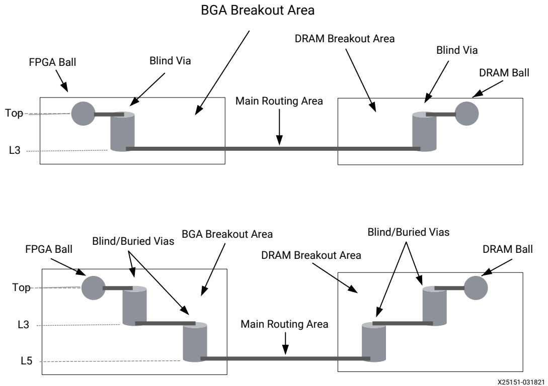
Figure 59: Examples of Stripline Routing for HDI LPDDR4 Signals
