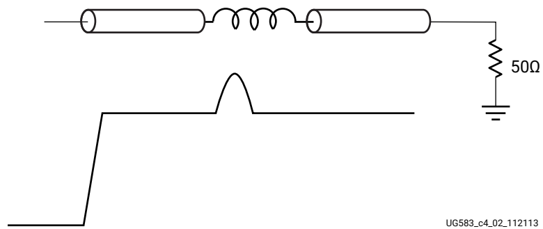
Figure 228: TDR Signature of Series Inductance
