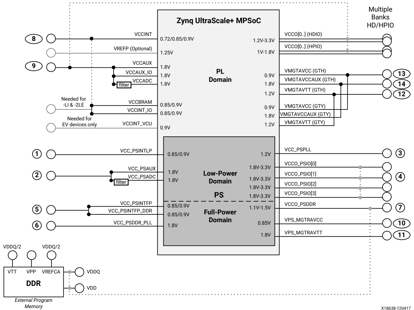
Figure 8: Full Power Domain Flexibility Consolidation
