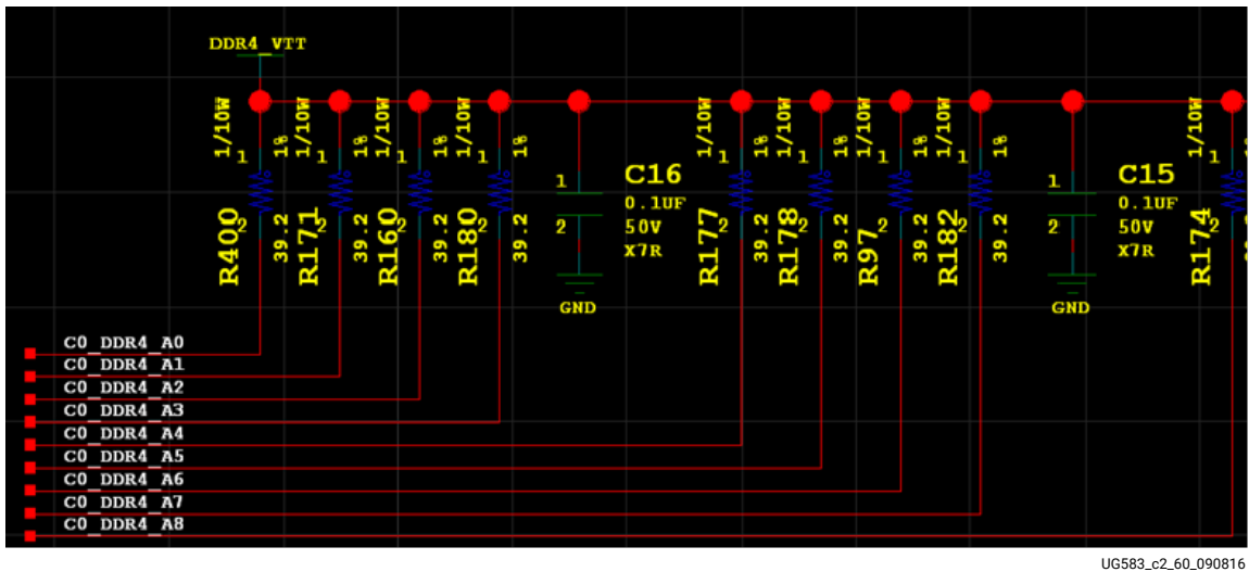
Figure 23: Schematic Example of VTT Resistor and Capacitor Connections
