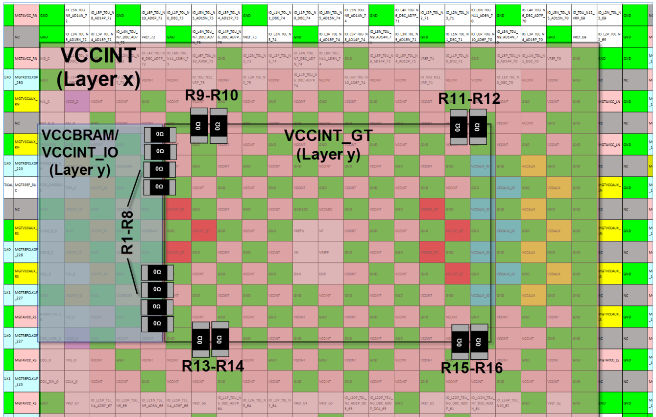
Figure 194: Layout Migration Example for Migration to VU27P/VU29P-2LE
