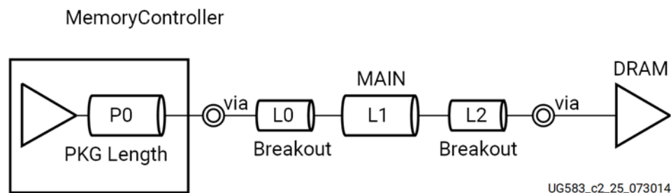
Figure 35: Data Signals Point-to-Point for DDR4 SDRAM
