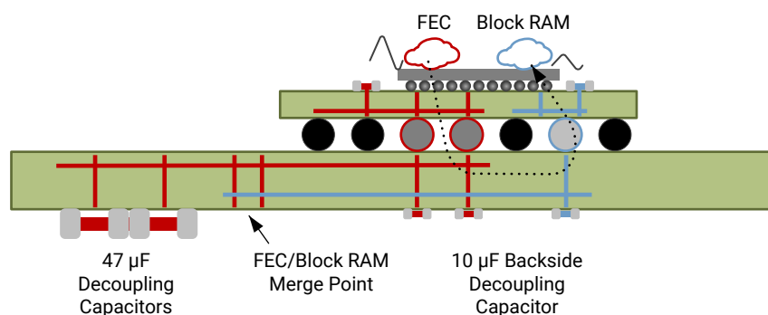
Figure 120: Recommended Plane Connection for V_{CCSDFEC} and V_{CCBRAM}
