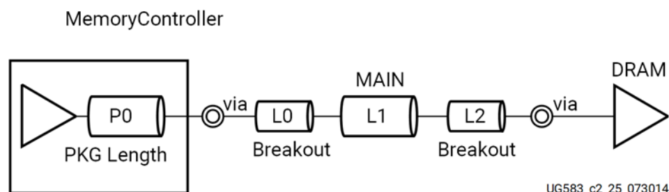
Figure 108: Data Signals Point-to-Point for DDR4 SDRAM
