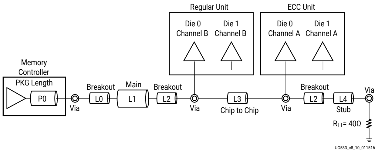
Figure 52: CA_B Address/Command Routing for LPDDR4 with ECC
