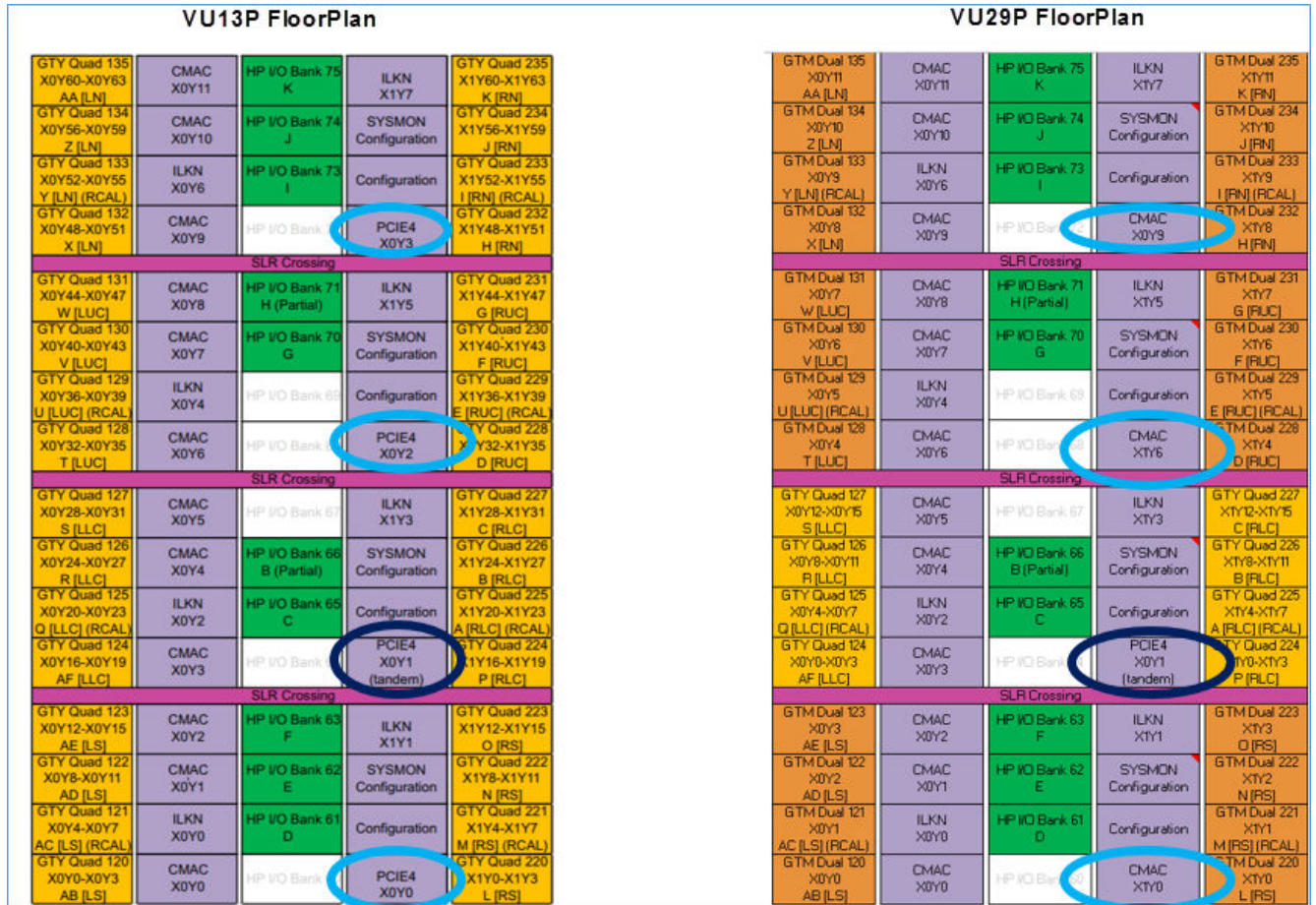
Figure 198: VU13P Floorplan with PCIe/GTY versus VU29P Floorplan with CMAC/GTM
