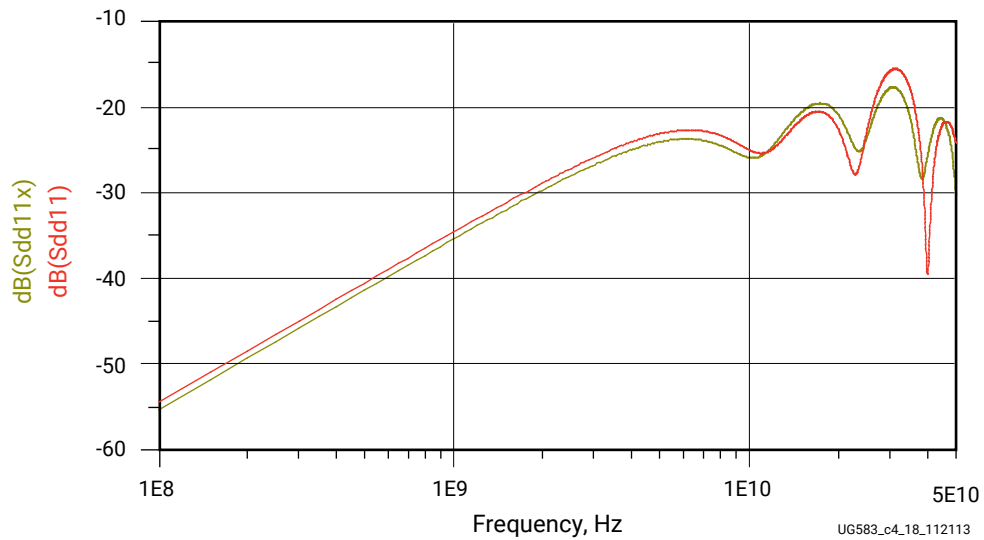
Figure 245: Simulated Phase Response of 45 Degree Bends with Jog-Outs
