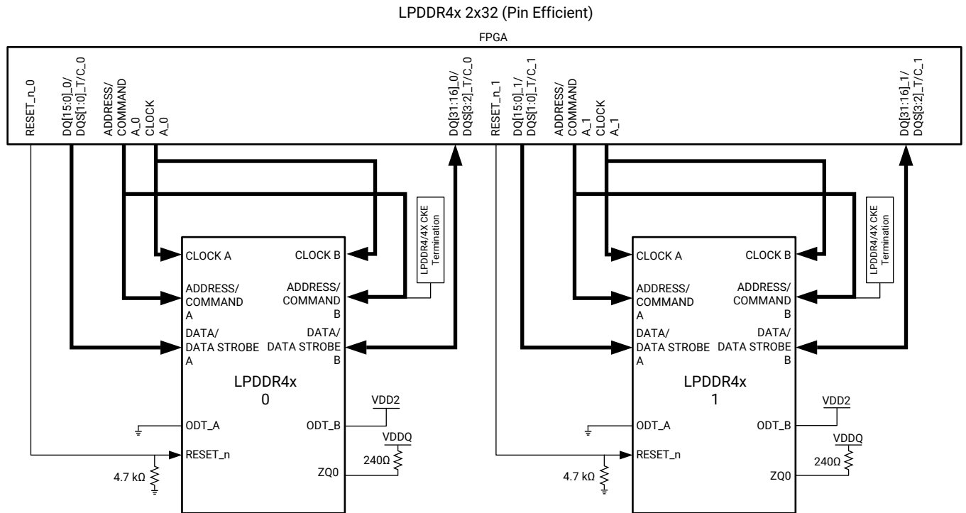
Figure 118: Connections for a Pin Efficient 2x32 LPDDR4x Interface
