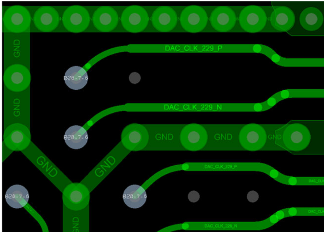
Figure 144: Layer 6 for Clock Routes
