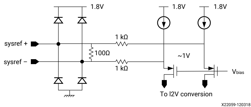
Figure 136: Analog_SYSREF Receiver Equivalent Circuit
