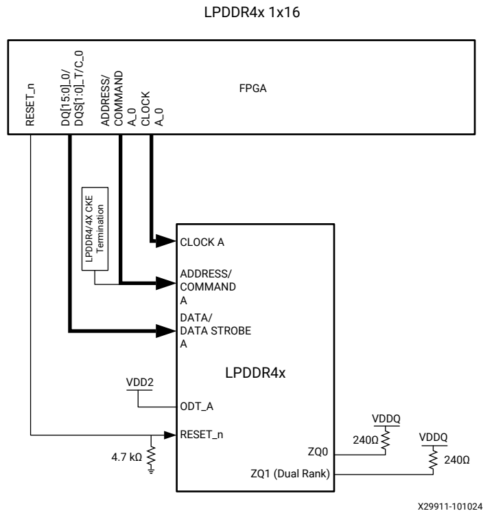
Figure 117: Connections for a 1x16 LPDDR4x Interface
