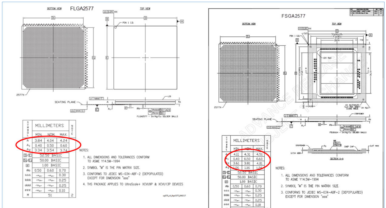
Figure 195: Package Dimension Differences between FLGA2577 and FSGA2577
