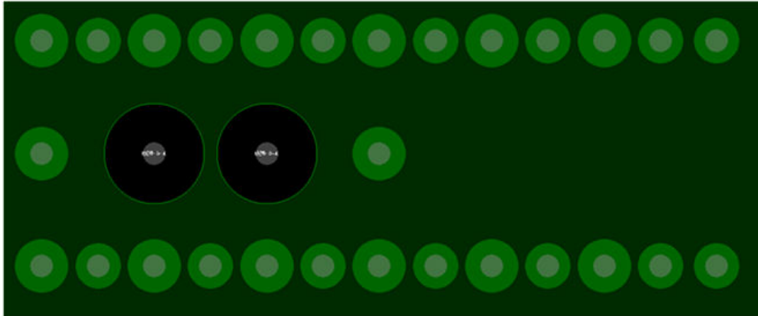
Figure 141: Layer 3 in BGA Area for DACs/ADCs
