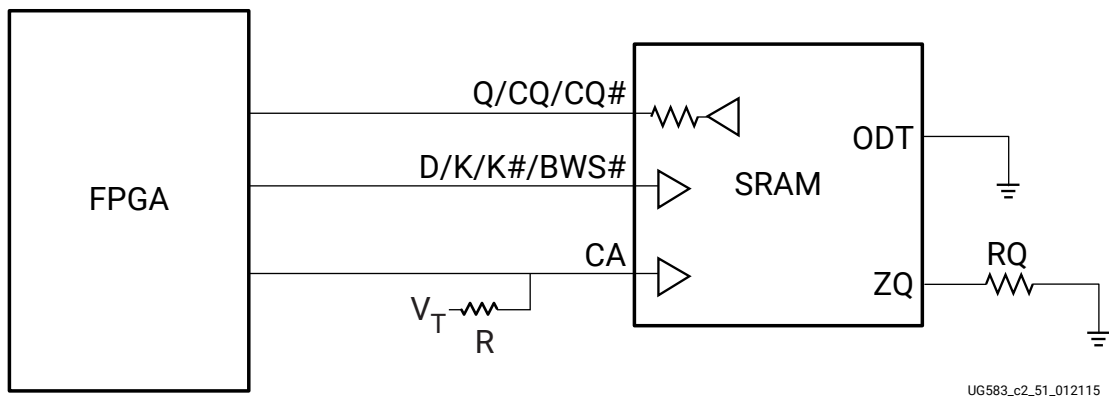
Figure 78: Design Example for Single QDR II+ SRAM Device
