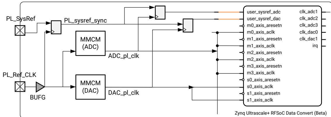
Figure 137: PL_SYSREF Capture
